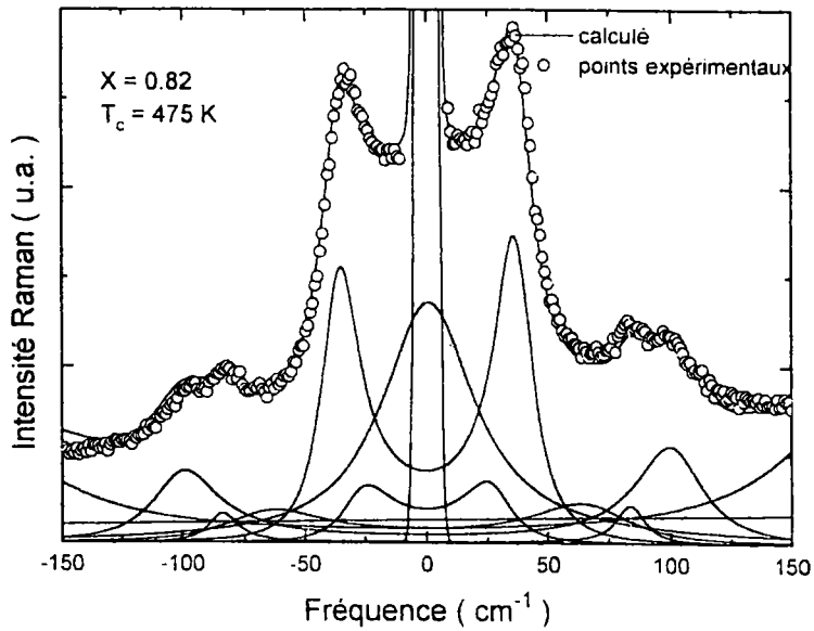
Spectre Raman de \text{AgTa}_{0.18}\text{Nb}_{0.82}\text{O}_3 à T_c=475 \text{ K} .
