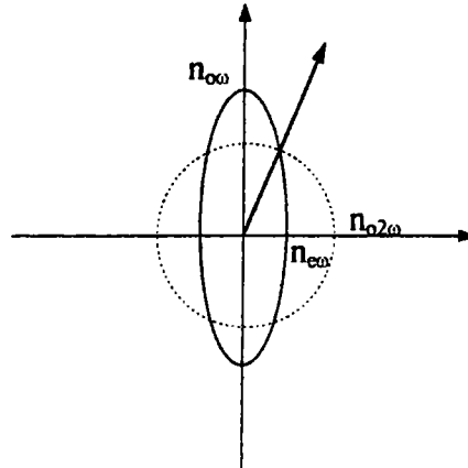
Accord de phase de type (ee-o) Figure III.3
