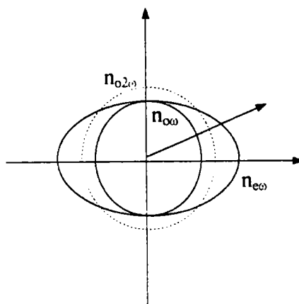
Accord de phase de type (oe-o) Figure III.4
