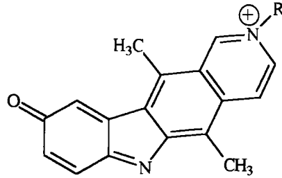
Quinone - imine
