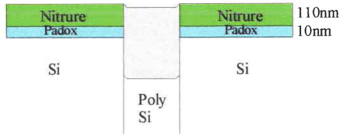
Fig.IVC.1 : Structure "Array"
