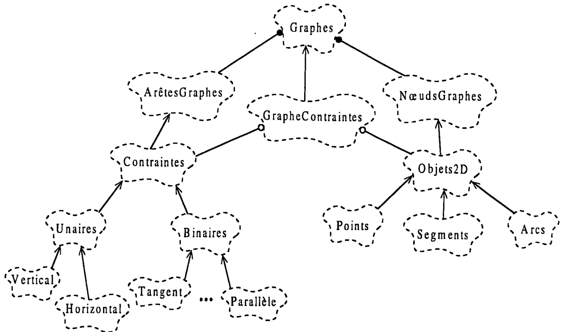
Figure B.1. Diagramme des classes
