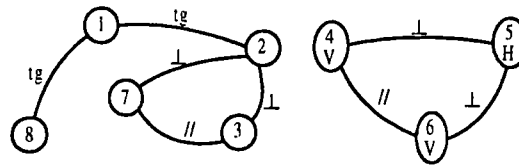
Figure 2.5. Graphe complet
