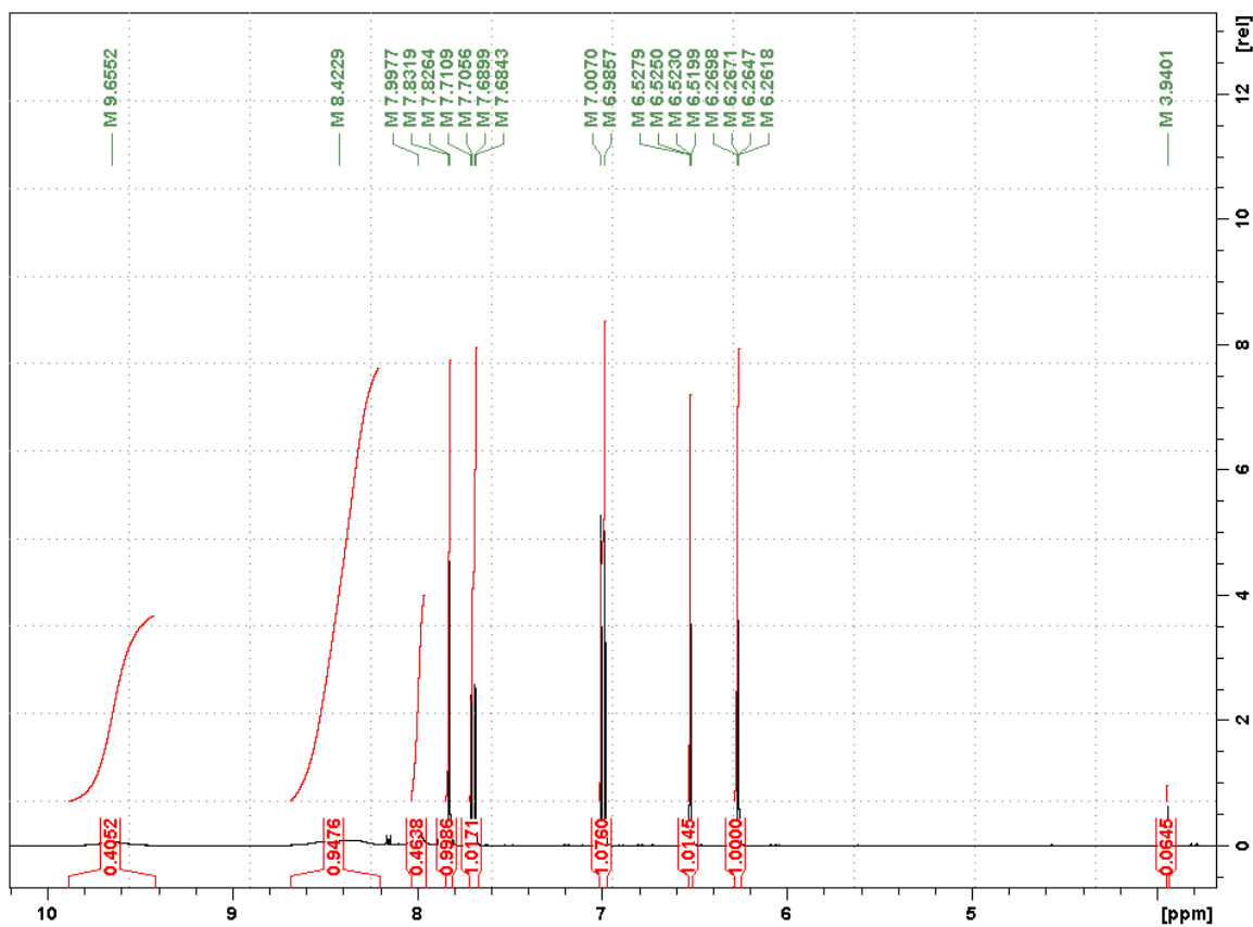
Figure 33: ^1\text{H} spectrum of compound N-2 in acetone d_6 at 400 MHz.
