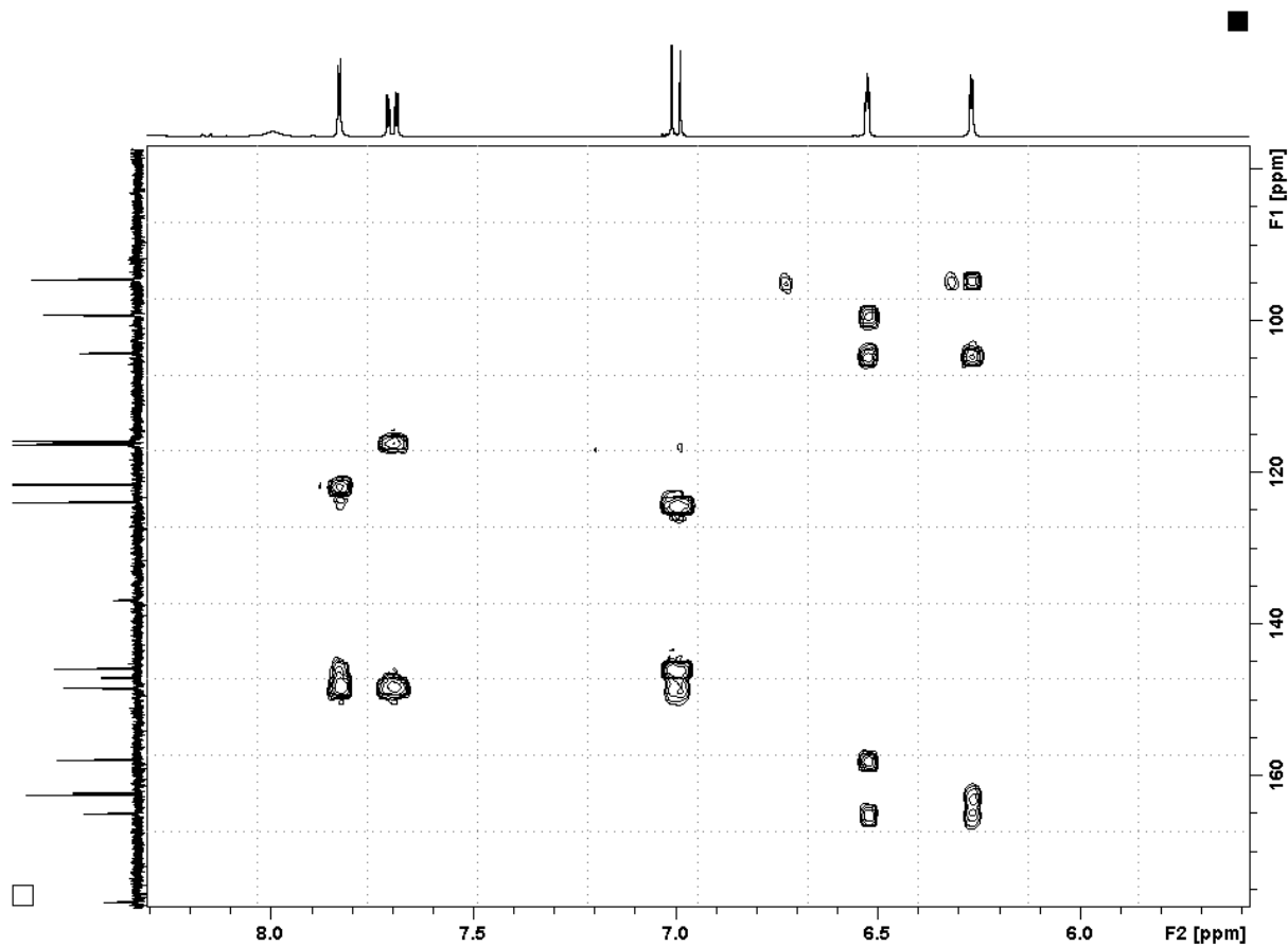
Figure 37: HMBC correlation of compound N-2.
