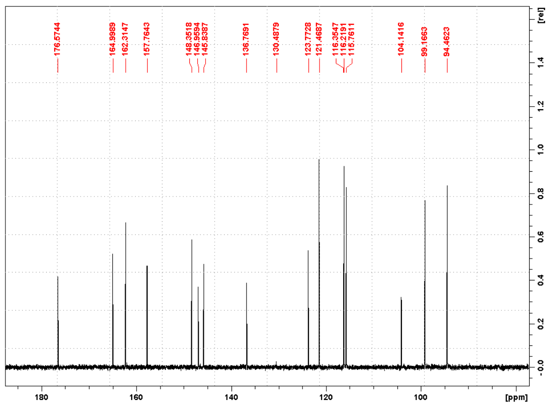
Figure 34: ^{13}\text{C} spectrum of compound N-2 in acetone d_6 at 100.6 MHz.
