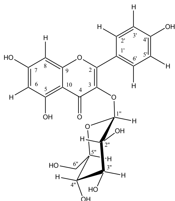
Figure 32: Structure of kaempferol-3-glucoside or astragaloside.
