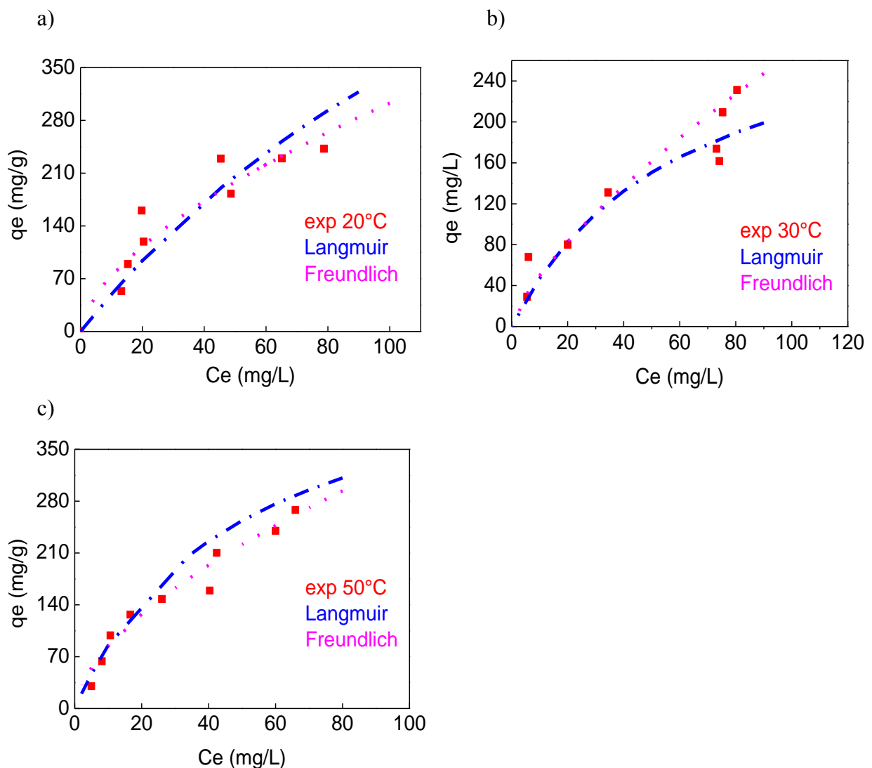
Figure 75: Experimental IBU adsorption isotherms at 20°C (a), 30°C (b) and 50°C (c) onto AC-HTC-240 presenting the fitting of Langmuir and Freundlich models to the experimental data
