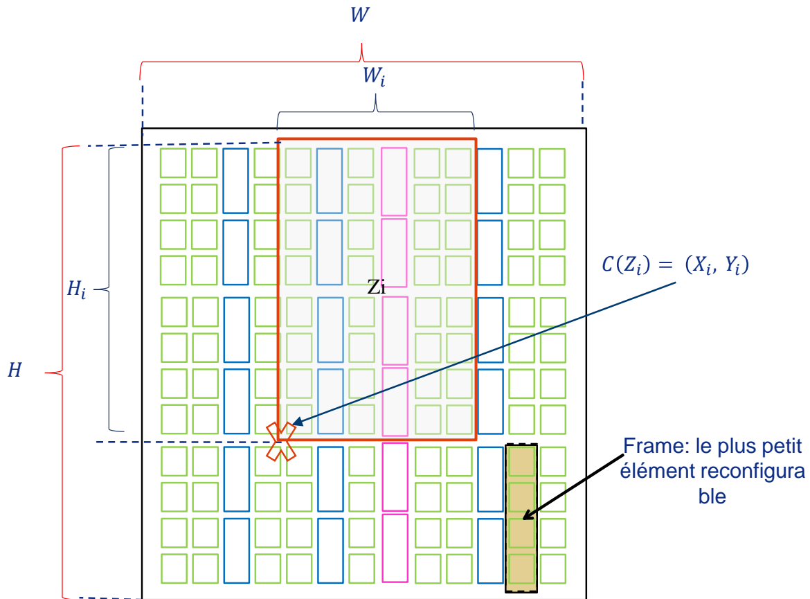
FIGURE 3.1 – Exemple de floorplanning
