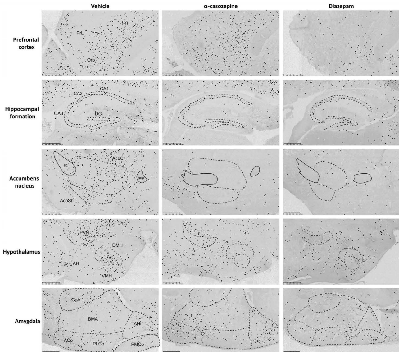
Fig. 5. Photomicrographs illustrating the effect of the vehicle, \alpha -CZP (1 mg/kg, i.p.), and diazepam (1 mg/kg, i.p.) on anxiety-induced c-Fos immunoreactivity in the prefrontal cortex (lateral 0.12 mm), hippocampal formation (lateral 0.48 mm), accumbens nucleus (lateral 0.84 mm), hypothalamus (lateral 0.12 mm) and amygdala (lateral 2.52 mm). Images followed the procedure as described in Fig. 2: green channel was extracted and images were inverted; black dots correspond to the c-Fos positive neurons extracted by ImageJ, using the Find Maxima function. Scale bar: 500 \mu m. Cg: cingulate cortex; PrL: prelimbic cortex; Orb: orbital cortex; CA1: field CA1 of hippocampus; CA2: field CA2 of hippocampus; CA3: field CA3 of hippocampus; DG: dentate gyrus; AcbC: accumbens nucleus, core; AcbSh: accumbens nucleus, shell; aci: anterior commissure, intrabulbar; acp: anterior commissure, posterior; AH: anterior hypothalamic nucleus; DMH: dorsomedial hypothalamic nucleus; PVN: paraventricular hypothalamic nucleus; VMH: ventromedial hypothalamic nucleus; Aco: anterior cortical amygdaloid nucleus; AHI: amygdalohippocampal area; BMA: basomedial amygdaloid nucleus; CeA: central amygdaloid nucleus; PLCo: postlateral cortical amygdaloid nucleus; PMCo: posteromedial cortical amygdaloid nucleus.
