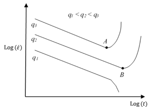
Figure 1.11 Typical relationship of creep strain rate with time under different stress level in undrained creep (after Zhu, 2007)
