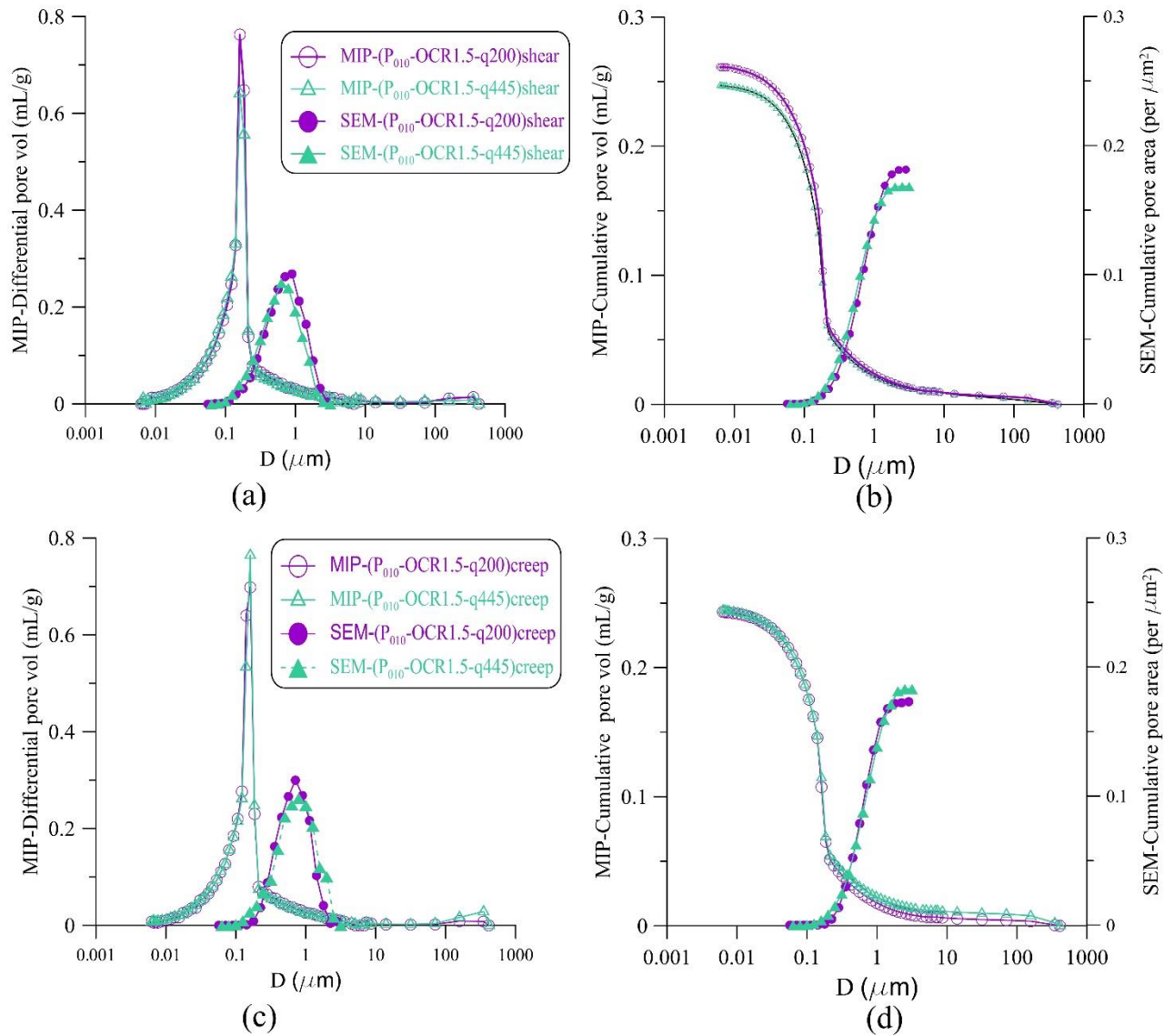
Figure 4-11 Evolution of pore area for tests with OCR=1.5: (a) (b) shear tests; (c), (d) creep tests
