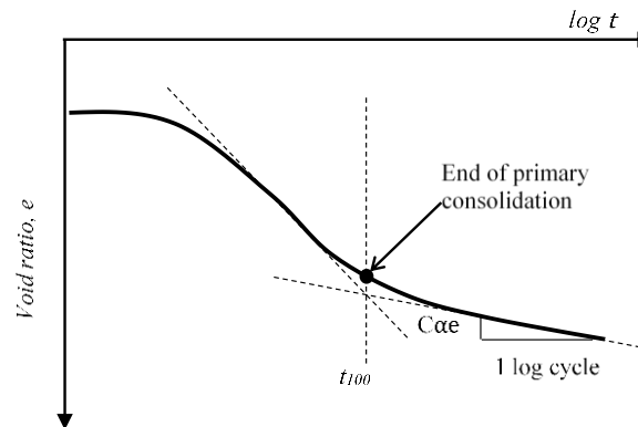
Figure 1.3 Identification of secondary compression coefficient
