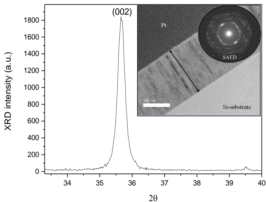
Fig. (5.14): XRD of (1.5% Ce, 1% Yb) co-doped Al(O)N sample. Inset: corresponding TEM and SAED images.
