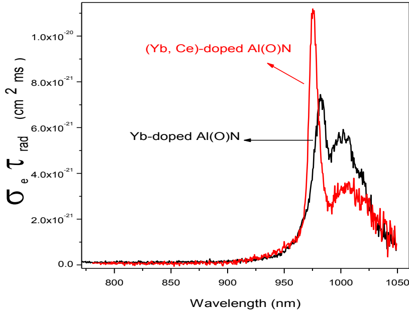
Fig. (D.1): The calculated \sigma_e \tau_{rad} parameter as a function of wavelength.
