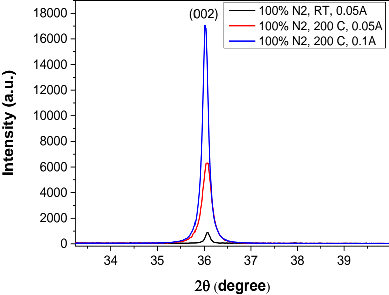
Fig (3.5): XRD of AlN samples deposited at 100% N 2 and different target current and substrate temperature.
