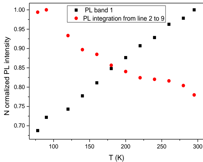
Fig. (5.12): Normalized PL as a function of temperature for band number 1 and integrated intensity for lines from 2 to 9 in fig (5.10).
