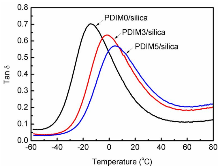
Figure 4-11. Temperature dependence of loss tangent ( \tan\delta ) for PDIM/silica nanocomposites.
