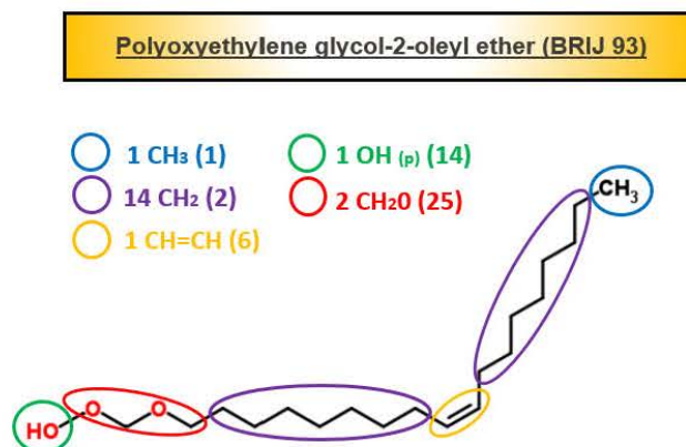
Fig. 3.11 Group assignments and molecular properties for surfactants included in the cartography.
