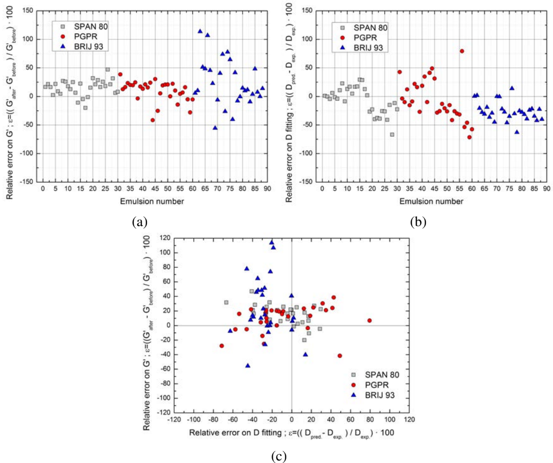
Fig. 4.17 a) Relative errors in storage moduli ( G' ) before and after release. b) Relative errors between predicted D_{\text{pred}} and experimental D_{\text{exp}} diffusion coefficients ( D ). c) Jointly representation of relative errors concerning G' and D .
