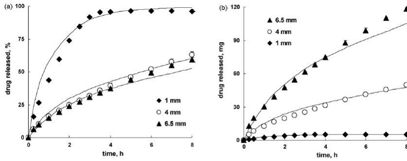
Fig. 1.20 Practical application of the 'sequential layer model': Theoretically predicted effects of the initial tablet radius on the release patterns of theophylline from HPMC-based matrix tablets in phosphate buffer pH 7.4 and experimental verification: (a) relative amount of drug released and (b) absolute amount of drug released versus time (37°C), initial tablet height = 2.6 mm, initial tablet radius indicated in the figures, 50% (w/w) initial drug loading) (curves: predicted values, symbols: independent experimental data). Taken from [9].
