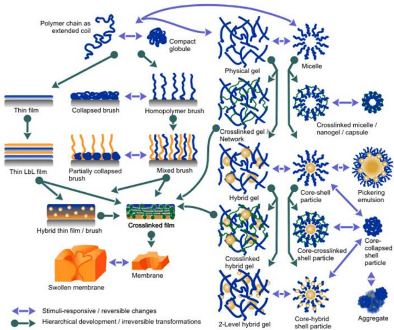
Fig. 1.10 Stimuli-responsive nanostructures based on polymers, colloids and surfaces Taken from [6].
