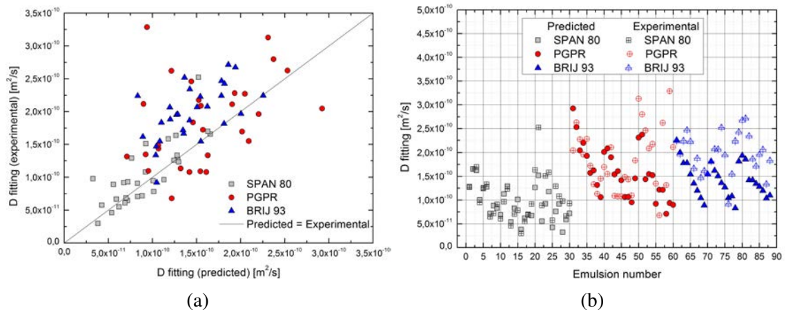
Fig. 4.15 a) Comparison of fitted diffusion coefficients of experimental curves versus predicted ones. b) Comparison of fitted coefficient values per sample.
