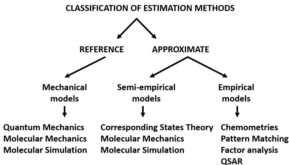
Fig. 1.4 Classification of property estimation methods. Adapted from [1].
