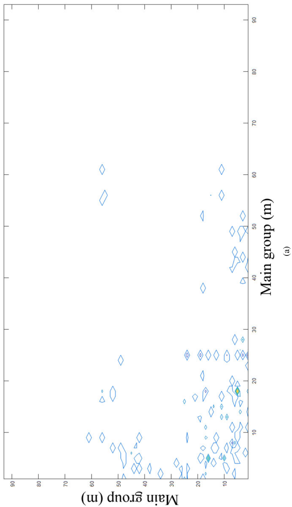
Fig. A.7 Top view of c_{fm} parameter matrix from Modified UNIFAC (Dortmund). Constantinescu et Grmehling (2016).
