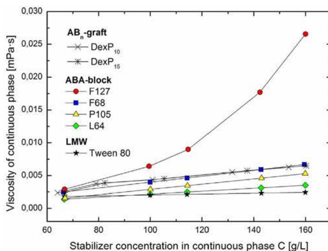
Fig. 4. Viscosity of continuous phases prior emulsification. Each point represents the initial concentration of stabilizer in the continuous phase at a given \phi (from left to right: 0.850; 0.900; 0.913; 0.930 and 0.938).
