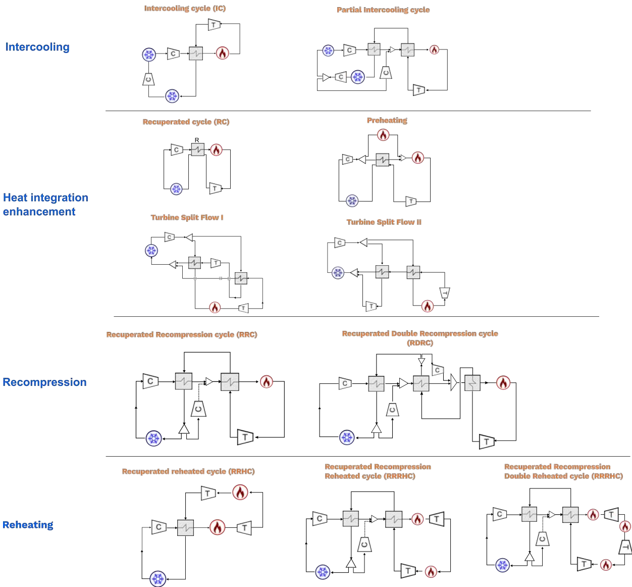
Figure 5.1: Classification of individual process modifications of SC-CO 2 Brayton cycle taken into account in the superstructure SS2 (Angelino, 1968; Mecheri and Le Moulec, 2015; Crespi et al., 2017)
