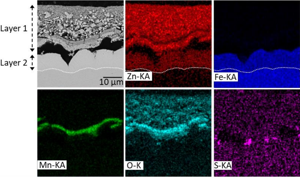
Figure 65: Cross-sectional SEM micrograph (BSE mode) and SEM-EDS elemental mapping of Zn-Mn coatings heat treated to 900 °C in a furnace heated in air; cross-sections carried out on white areas of the specimens (Figure 59).
