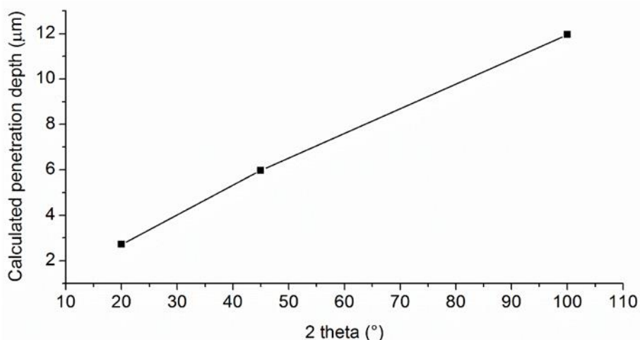
Figure 47: X-ray penetration depth in a Zn-Mn coating calculated using the AbsorbDX software and by considering a density of 7.104 \text{ g/cm}^3 (JCPDS n°01-077-2965), a wavelength of 1.5406 \text{ \AA} , a contribution of 90 % to the diffracted beam and in the Bragg condition.
