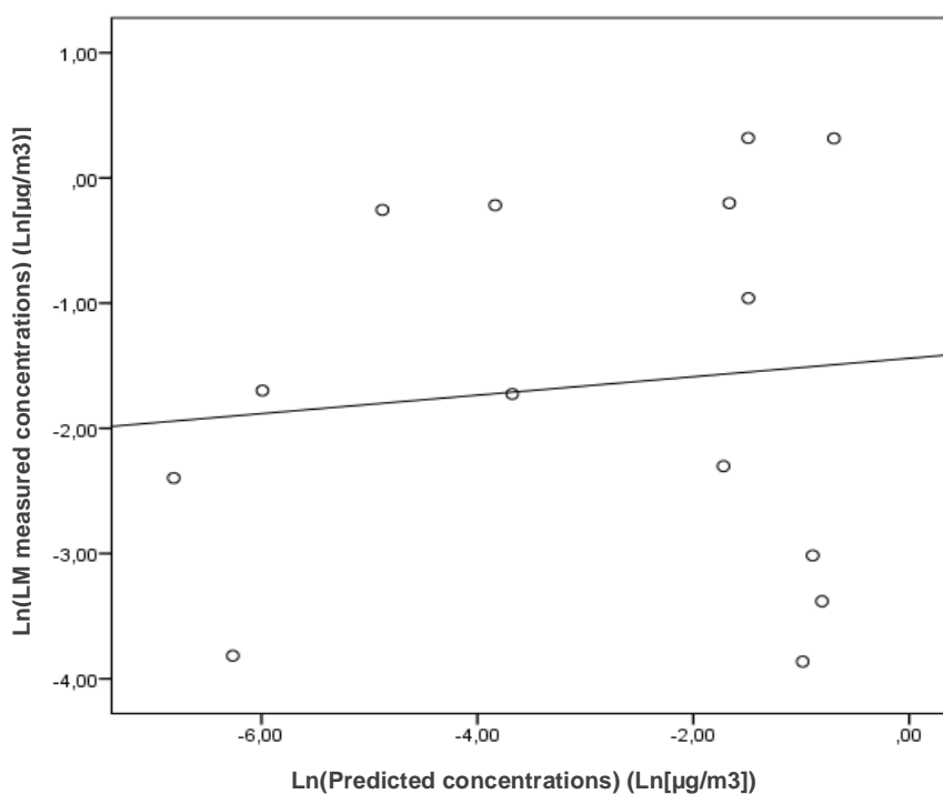
Figure 2.27: Linear regression of the Ln(Predicted TMEs concentrations) against the Ln(LM of the measured of the TMEs concentrations) of the packaging job tasks (FF for P3, P7 and P8)
