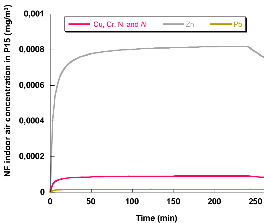
Figure 1.28: Modeled indoor air concentrations of Al, Cu, Ni, Cr, Zn and Pb in the NF of plastic injection molding (P15) during four-hour shift
