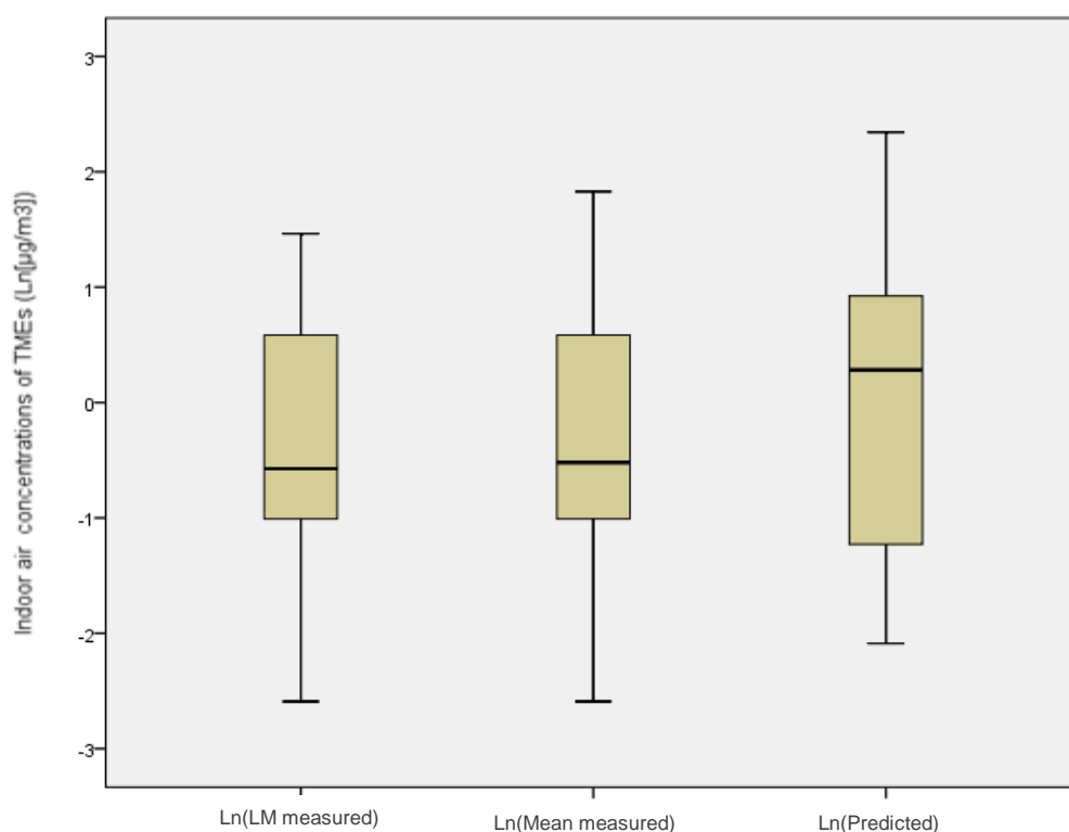
Figure 2.15: Distribution comparison of Ln(LM measured concentrations of the TMEs), Ln(Mean measured concentrations of the TMEs) and Ln(modeled TMEs concentrations) of welding job tasks (NF in P5 and P9)
