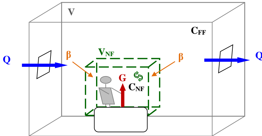
Figure iii: Near-Field, Far-Field model presentation; G : generation rate, Q : ventilation rate, \beta : inter-box air flow rate, V : air volume, V_{NF} : NF air volume, C_{NF/FF} : predicted concentration of the pollutant in the NF and FF, respectively
