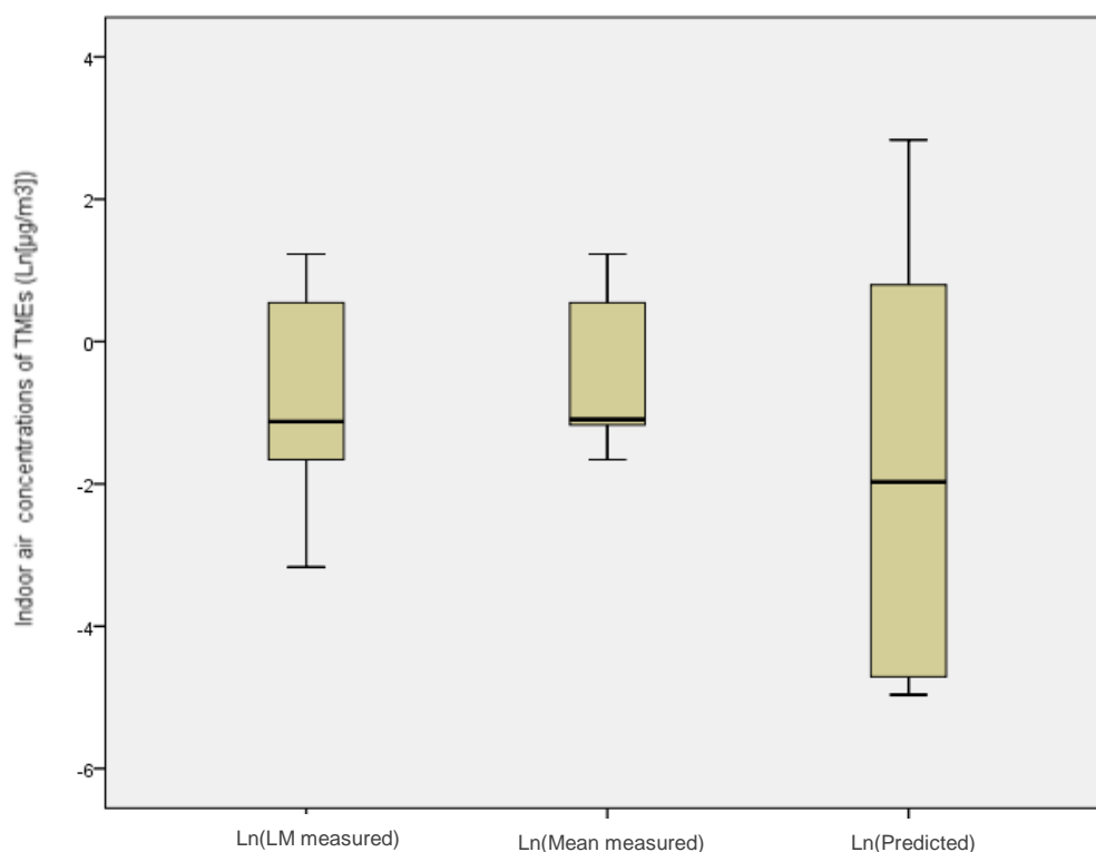
Figure 2.18: Distribution comparison of Ln(LM measured concentrations of the TMEs), Ln(Mean measured concentrations of the TMEs) and Ln(modeled TMEs concentrations) of welding job tasks (combined exposure in P16)
