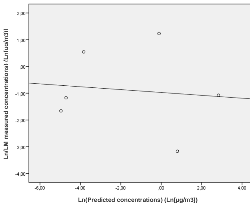
Figure 2.19: Linear regression of the Ln(Predicted TMEs concentrations) against the Ln(Mean of the measured of the TMEs concentrations) of welding job tasks (combined exposure in P16)
