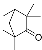
Fenchone
