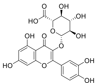
Quercétine-O-glucuronide
