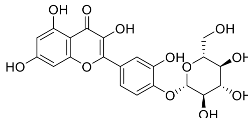
Spiraeoside
