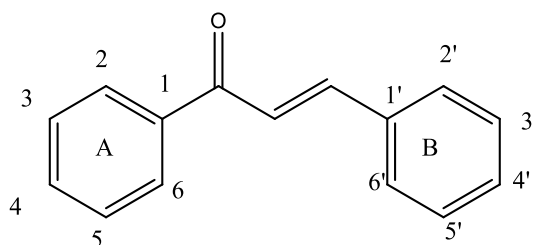
1,3-Diphényl-2-propen-1-one
