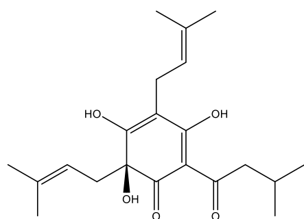
Humulone (alpha-acide).
