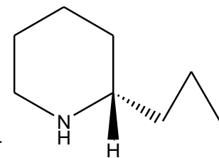
Coiine
