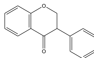
Isoflavonoids
