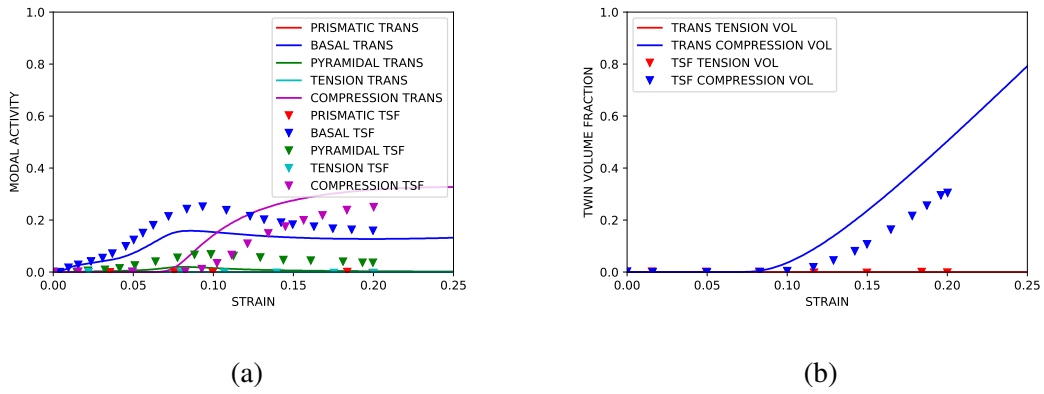
Figure 4.7: Simulated twin slip and secondary twinning activity under IPC compression compared to simulated results from [83]. (a) Simulated modal contributions to strain vs. strain. (b) Simulated twin volume growth vs. strain.
