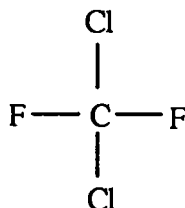
Figure II.4. Dichlorodifluoromethane
