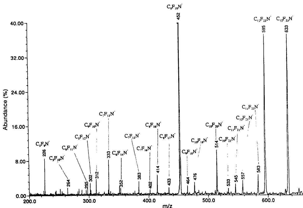
Figure IV.6. Negative ion mass spectrum obtained after laser-induced electron ionization of PFTBA (laser irradiance 10^8 W cm -2 ). The metal target was aluminum.
