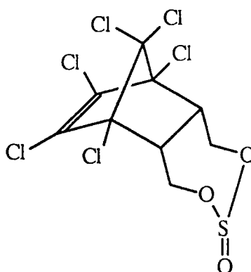
Figure II.6. Endosulfane
