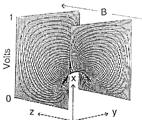
Figure I.6. Simulation plot of the trapping field equipotentials between both trapping plates at a 1 V potential. Ions are confined in the xy plane by the magnetic force.
