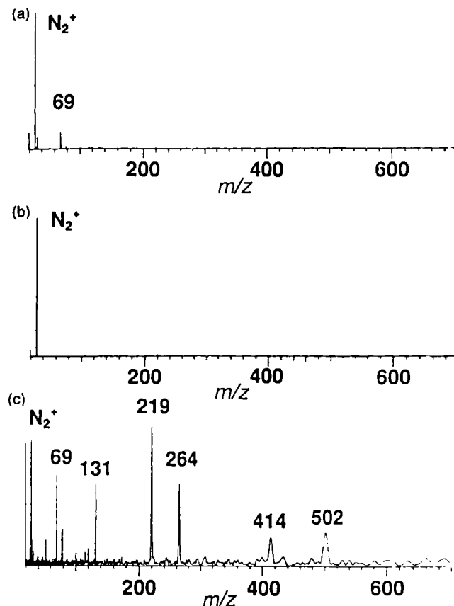
Figure III.5.4. (a) EI of PFTBA and air in source trap at 5 \cdot 10^8 Torr. (b) all ions below 1.55 MHz are ejected from the trap by double-resonance, leaving N_2^+ ions. (c) Excitation of cyclotron motion of the projectile ions through a cloud of PFTBA ionizes PFTBA by the IIII process (from ref. 24)
