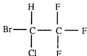
Figure II.5. Halothane
