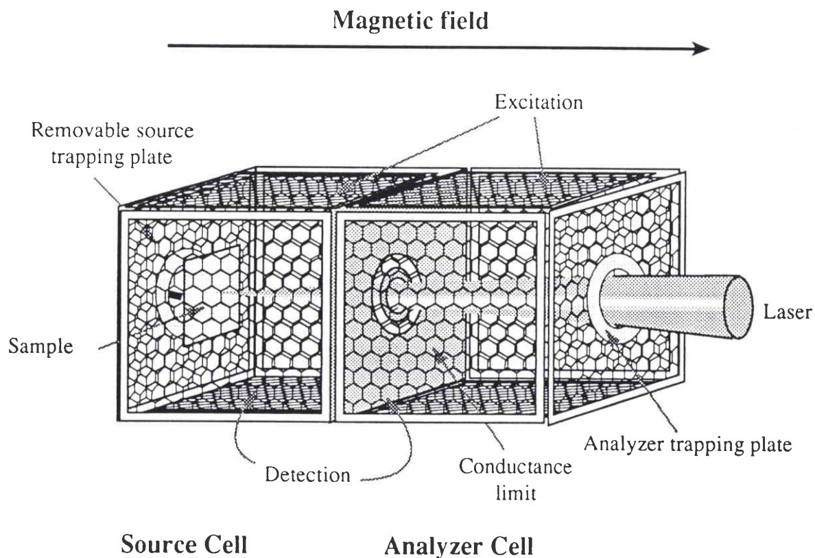
Figure II.2 : The double-cell (drawing taken from ref. 9).
