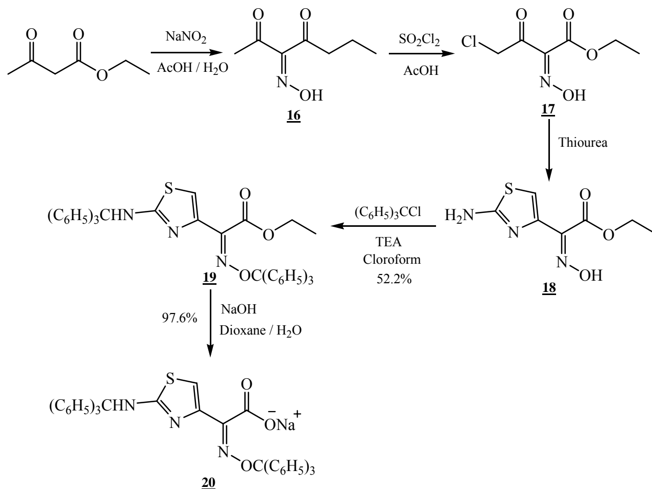
Scheme 15
