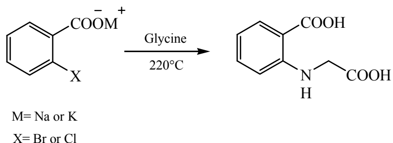
Scheme 28
