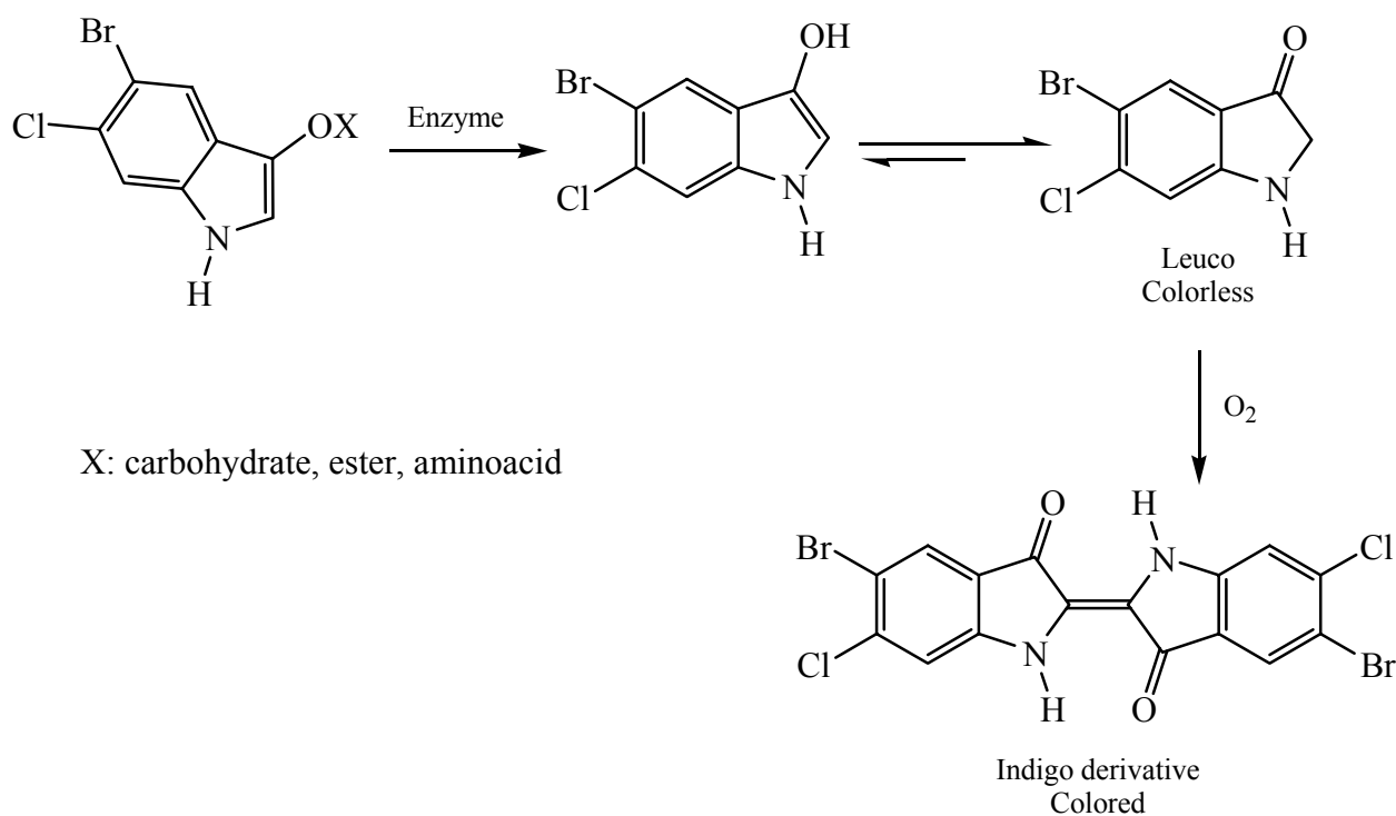
Scheme 22
