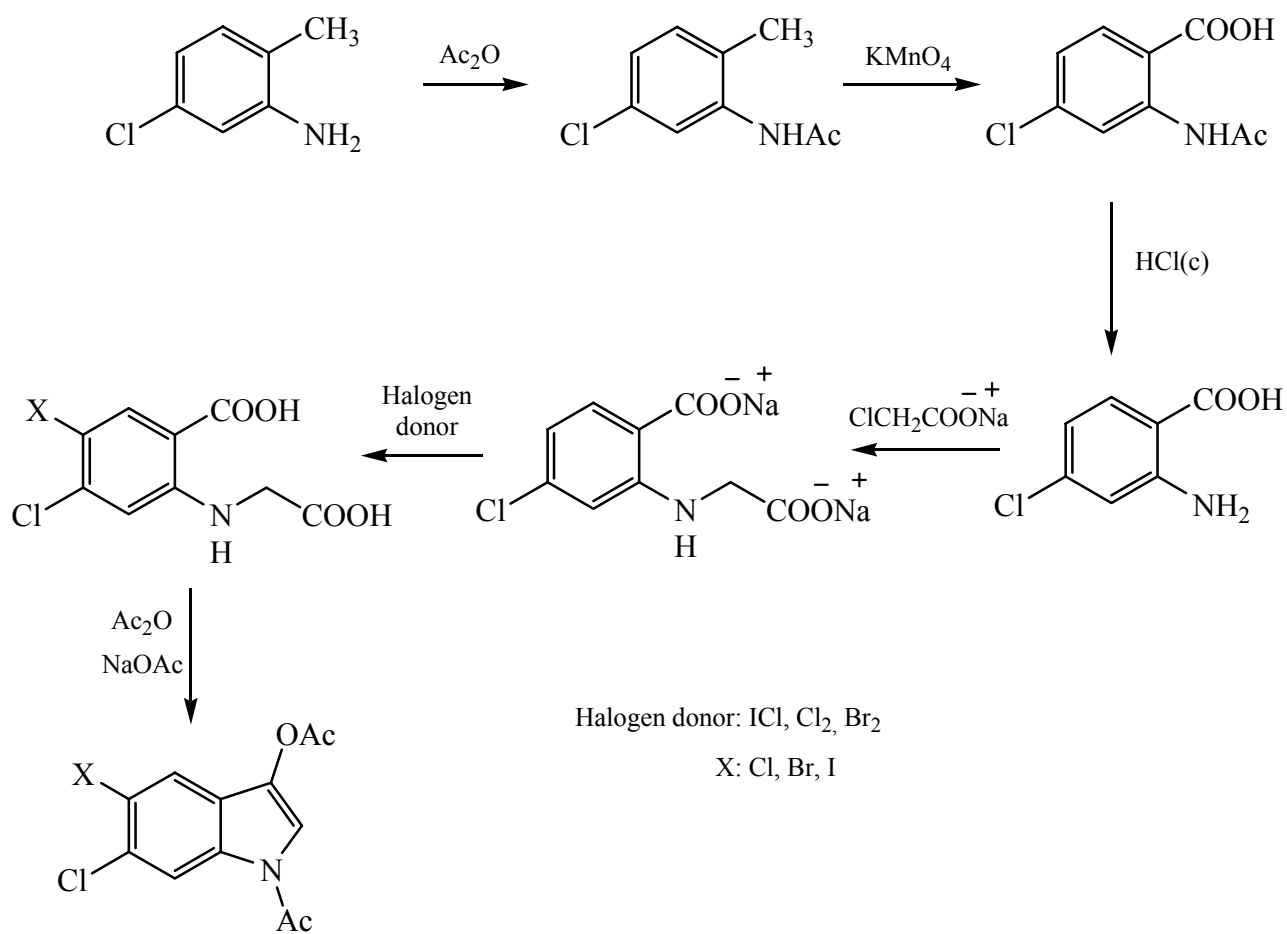
Scheme 25
