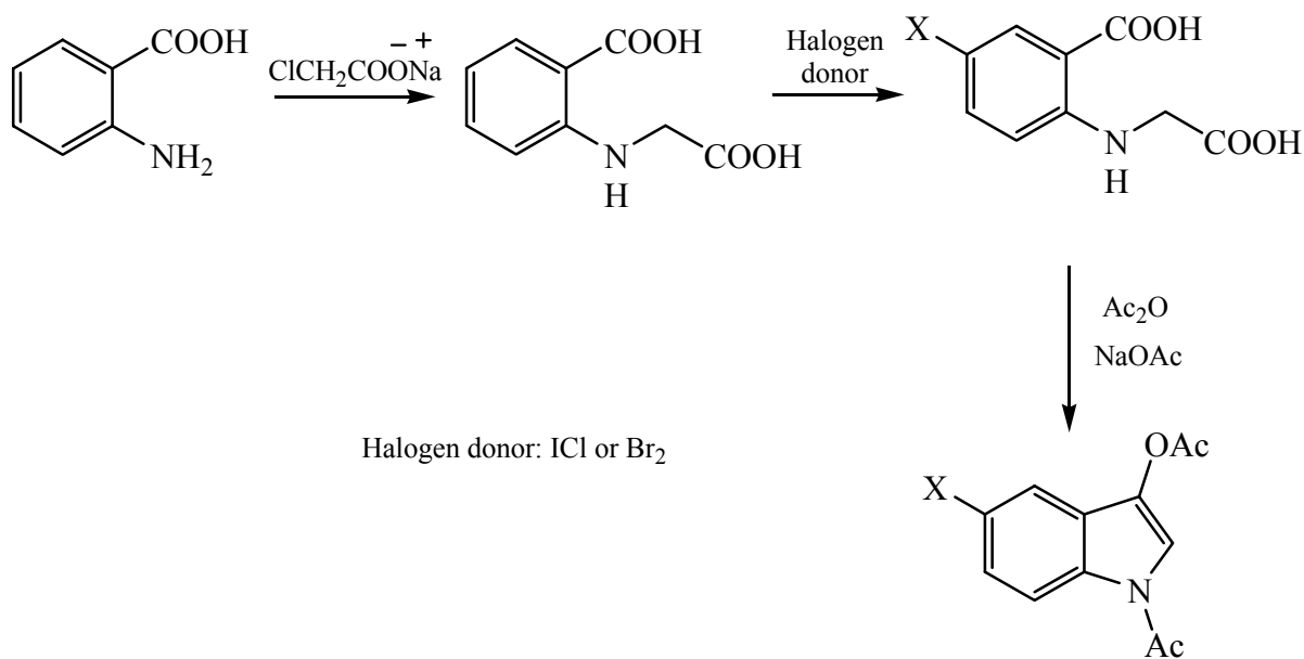
Scheme 26
