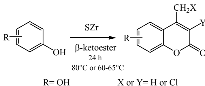
Scheme 18
