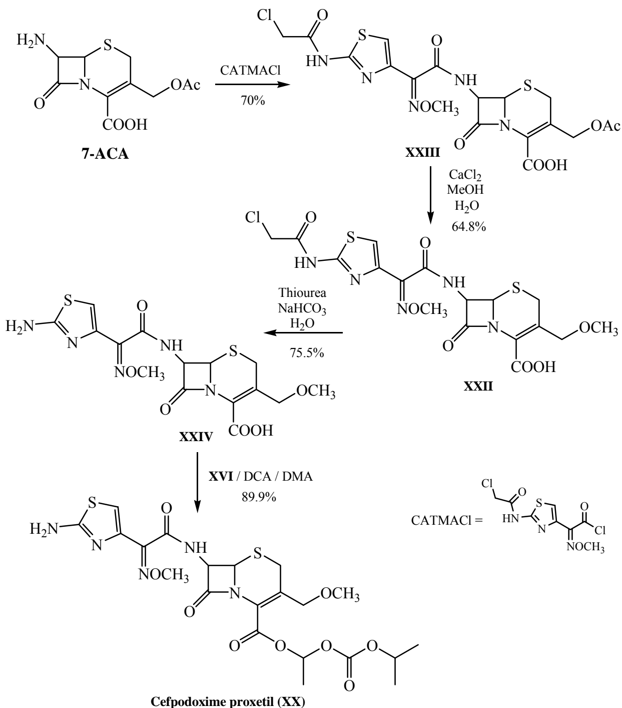
Scheme 10
