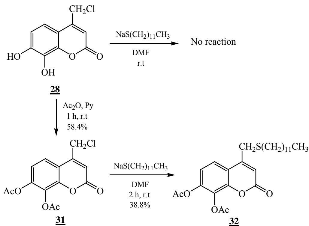
Scheme 19
