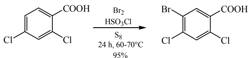
Scheme 30
