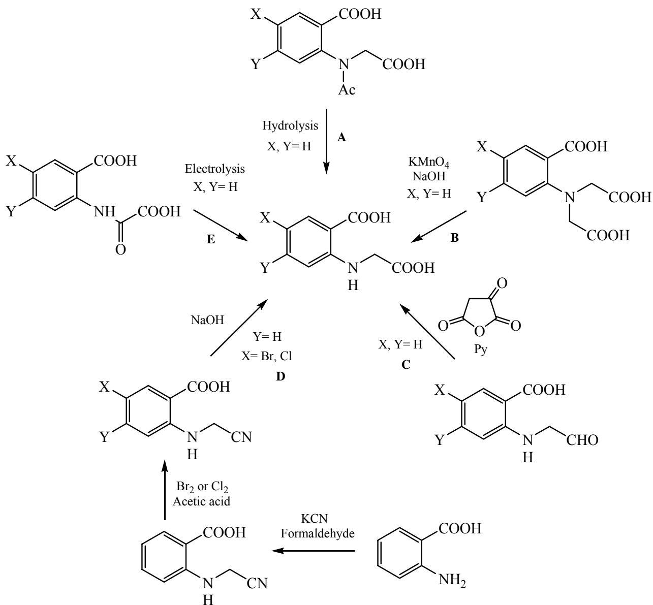
Scheme 27
