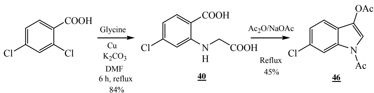
Scheme 29
