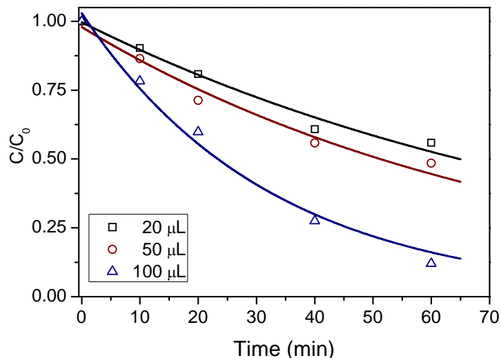
Figure 4.11 The effect of H 2 O 2 on the photocatalytic activity of hematite. The net volume of the reaction solution is 100 ml.
