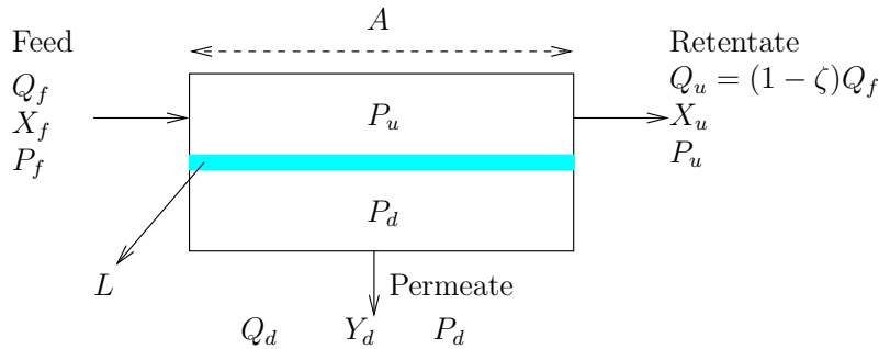
Figure 2.2: Notations of a conventional membrane-based gas separation process
