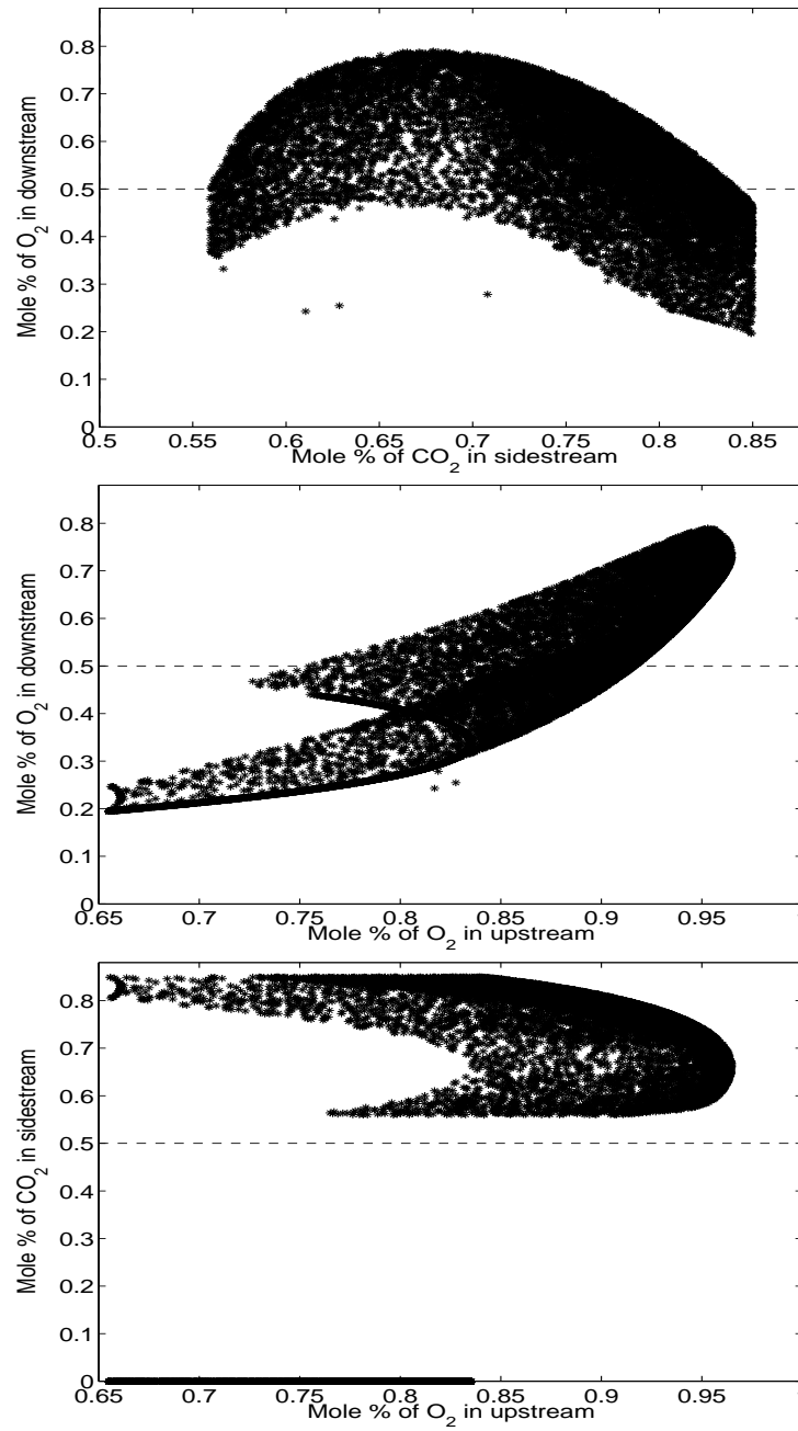
Figure 5.29: Relationship between mole fractions of \text{O}_2 in upstream, mole fraction of \text{CO}_2 in sidestream and mole fraction of \text{O}_2 in downstream. Initial mole fraction of \text{O}_2 or \text{CO}_2 is represented by dashed lines.
