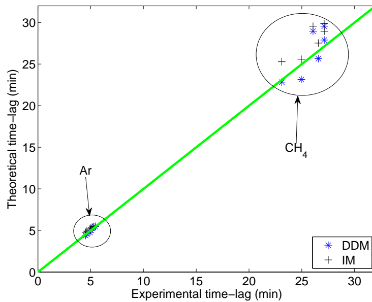
Figure 4.13: Comparison of experimental [Chiou and Paul, 1989] and predicted time-lags by different models for Ar and CH 4 in PEMA film at 35°C. (DDM = Dual Diffusion Model, IM = Immobilization Model).
