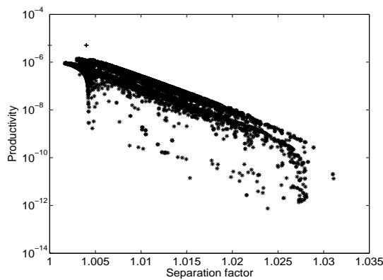
Figure 5.6: Comparison of separation performances for steady-state operations(+) and a short class process (*) with a \text{UF}_6 mixture. Test conditions in Tab. 5.7 for a membrane of 2 \text{ mm} .
