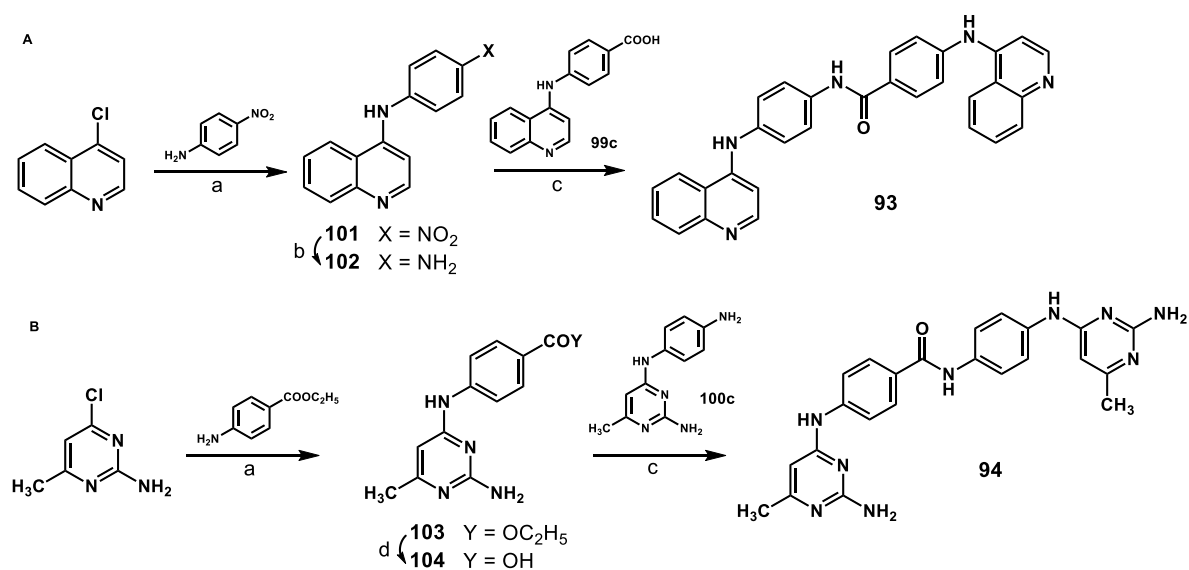
Scheme 16: Reagents and conditions: (a): 37% HCl, CH 3 CH 2 OH, 80 °C, 2 h; (b): stannous chloride dihydrate, 37% HCl, CH 3 CH 2 OH, 80 °C, 1 h; (c): (C 2 H 5 ) 3 N, PyBOP, anhydrous DMF, N 2 atmosphere, room temperature, 1 h; (d): 2 N KOH, CH 3 CH 2 OH.
