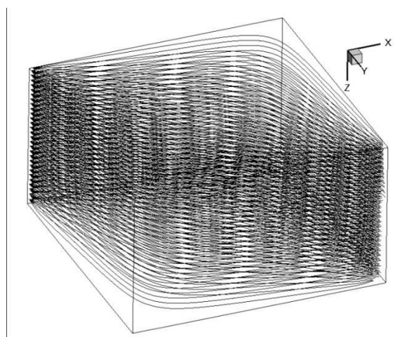
Figure 24- Streamline tracing in 3D geometry for isotropic permeability
