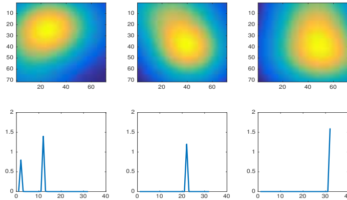
Figure 2.28: Example 4: abundance maps and endmembers of example 4.
