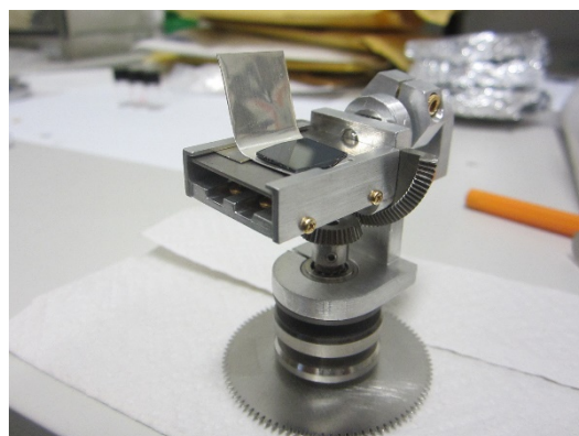
Fig. II-11: Experimental setup showing the sample holder for the sputter deposition of PS/PMMA on Ag foil
