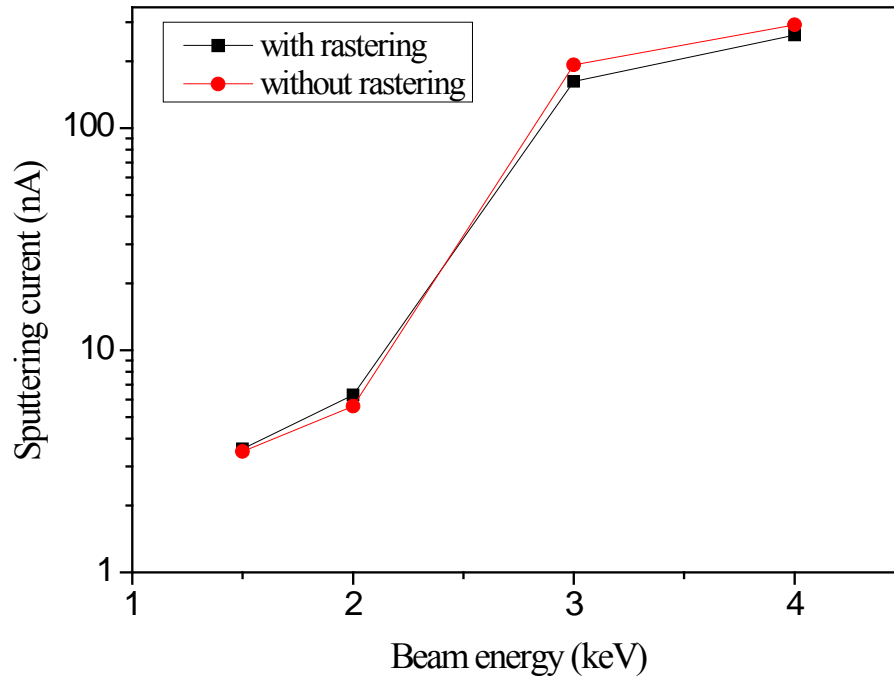
Fig. II-14: Variation of sputtering current with \text{Ar}^+ ion beam energy at 1 mA emission current
