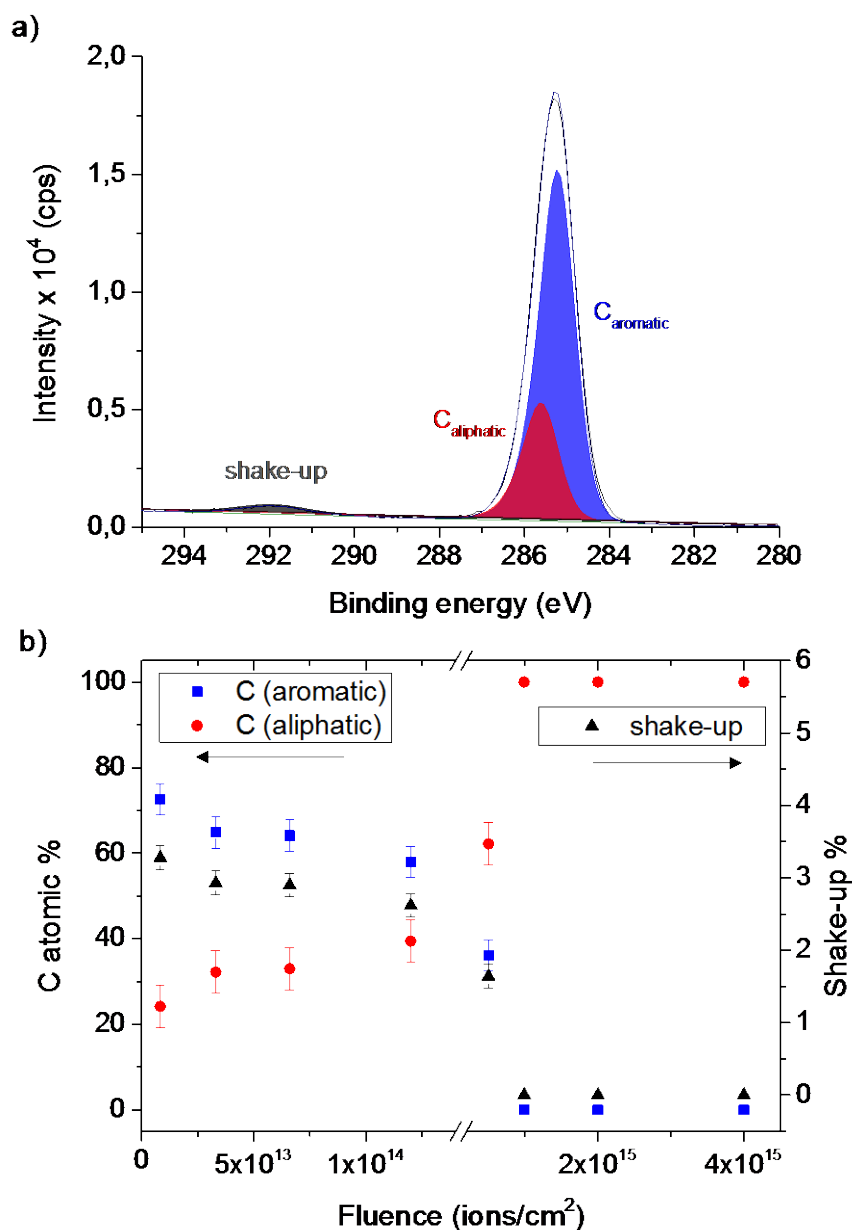
Fig. IV-14: a) XPS peak fit of the C 1s core level of bulk PS, b) Evolution of percentage values of C 1s core level of bulk PS as a function of the primary ion fluence for a total number of Ar + primary ions in the range 1.5x10 12 -8.9x10 13 .
