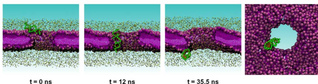
Figure 4.27: The process of siRNA transport, when U_m is above 0.5 V, in three frames corresponding to 0, 12, and 35.5 ns. In the last panel the top view clearly shows the anchoring interaction. The POPC headgroups are shown as mauve and violet beads, the tails as purple lines; sodium and chloride ions are colored in yellow and gray; siRNA is green
