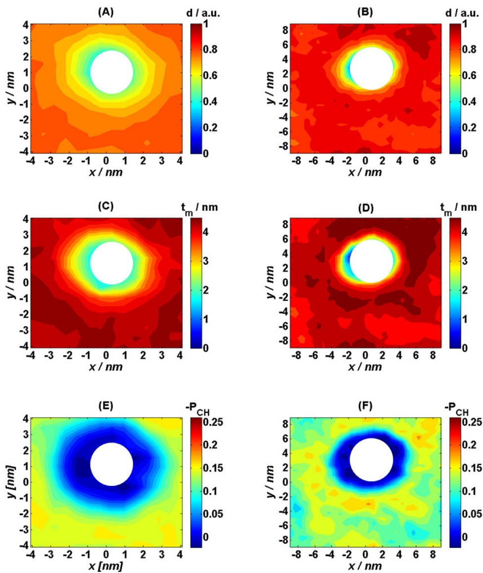
Figure 4.24: 2D spatial maps of the density d /a.u (A and B), thickness t_m /nm (C and D) and order parameter P_{CH} (E and F) estimated for the POPC-256 (A, C, E) and POPC-1024 (B, D, F) bilayers subject to \sim 500 mV
