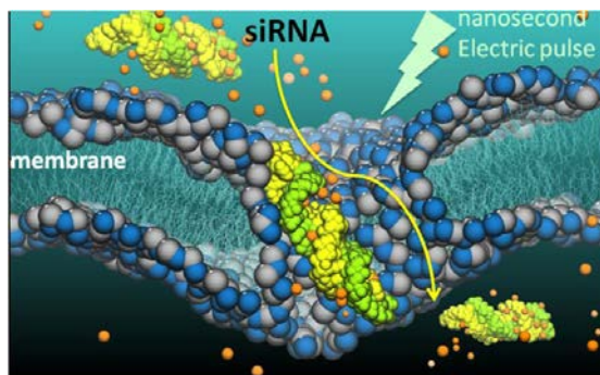
Figure 2.19: Molecular snapshots of the mechanism of electrotransfer of a double-stranded siRNA (shown as yellow and green spheres) through an aqueous pore (water omitted for clarity) within a POPC membrane (head groups shown as blue and gray spheres and hydrophobic tails as cyan lines) [42]
