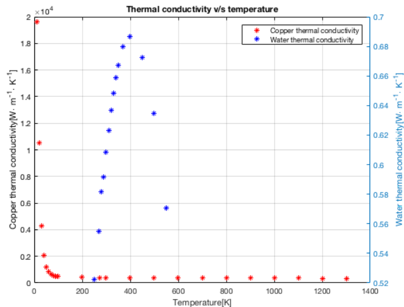
Figure 1.6: Thermal conductivity of copper and water v/s temperature [147]
