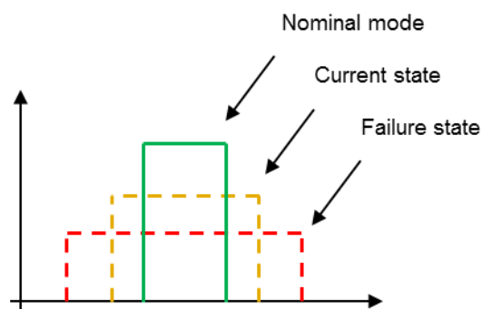
Figure 38: Histogram deviation type II
