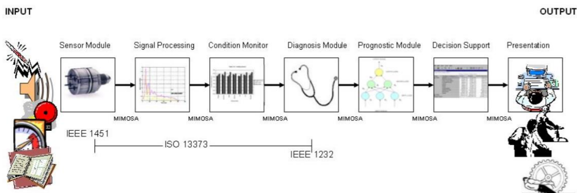
Figure 11: Sequential modules of CBM systems (Bengtsson, 2004)
