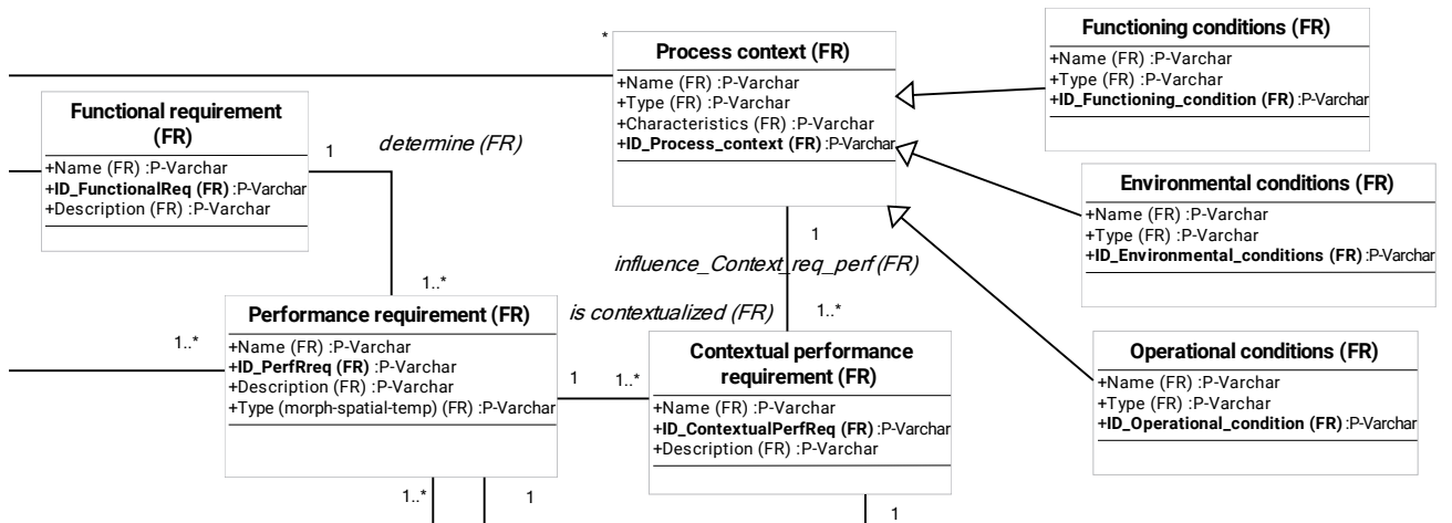
Figure 26: Extract of meta-model related on contextual concepts of knowledge
