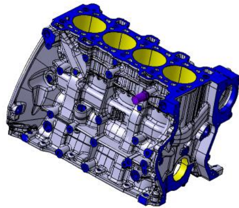
Figure 4: Renault engine cylinder-block
