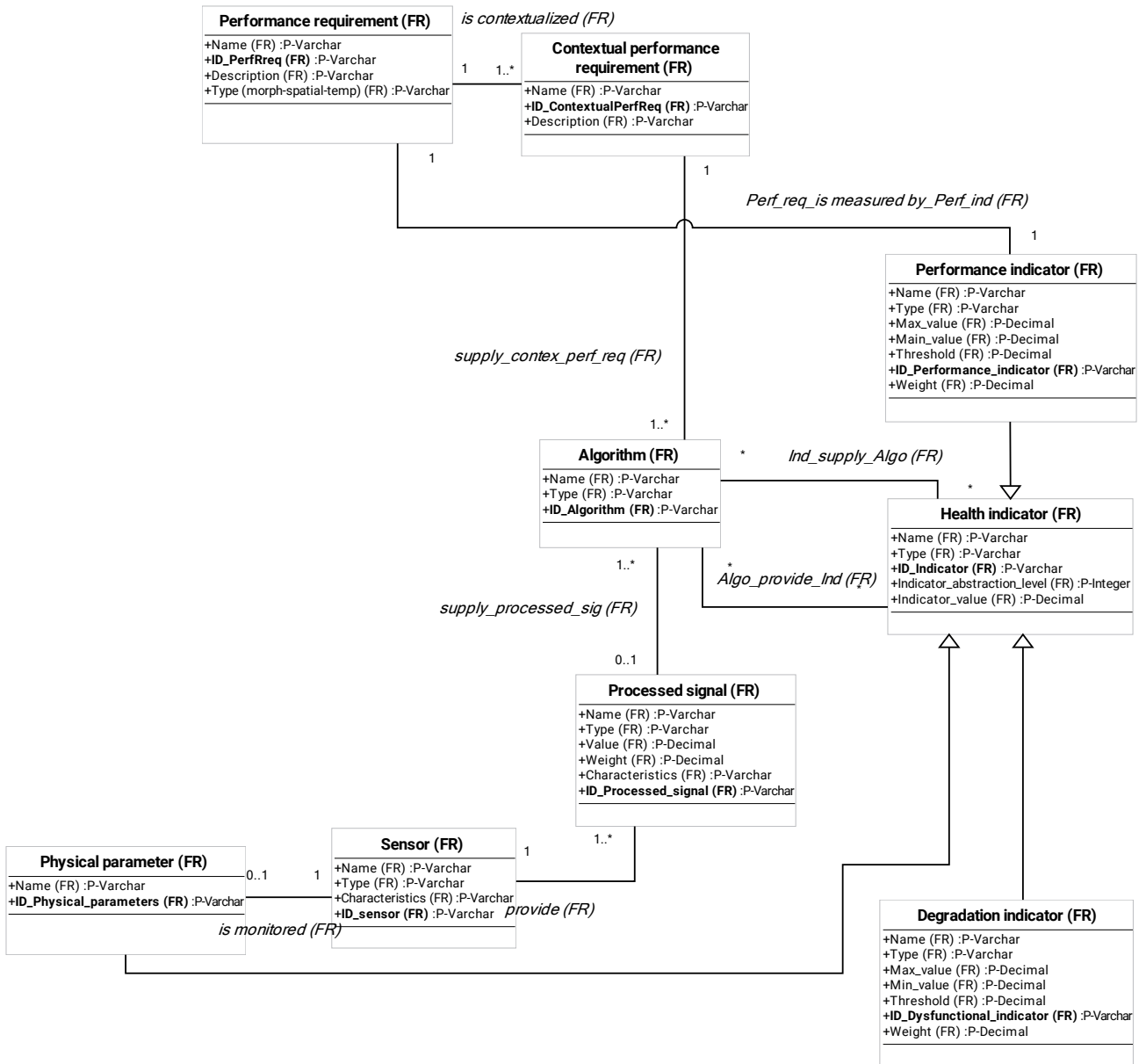
Figure 27: Extract of meta-model related on health indicator elaboration concepts of knowledge
