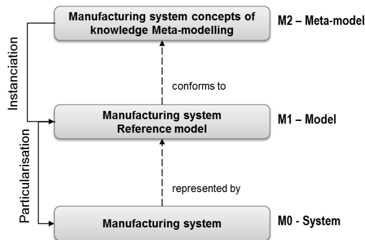
Figure 28: Meta-model instantiation framework
