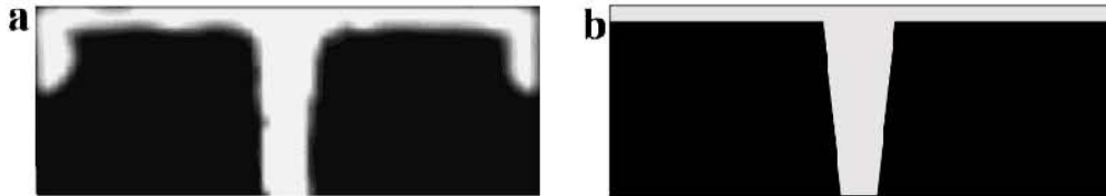
Fig. 6. Smoke configuration at t=23 s: (a) obtained by FDS, (b) obtained by the two-zone model (using Heskestad's plume model).
