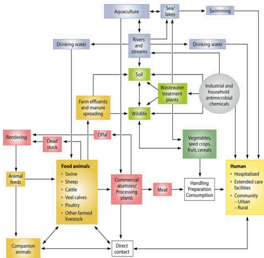
Figure 12. Dissemination routes of ARB and ARGs in the environment influenced by anthropogenic activities (source: Davies and Davies 2010).
