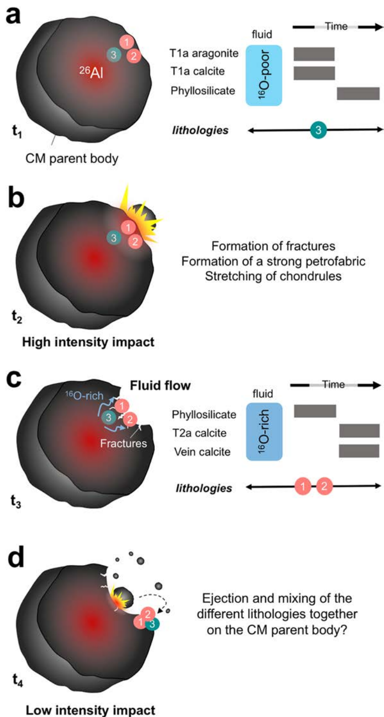
Fig. 14. Schematic representation of the thermal and deformation history of the CM parent body and the expected locations of the Boriskino lithologies at different times. (a) t_1 : precipitation of the Type 1a calcite and aragonite of lithology 3 by the decay of the ^{26}\text{Al} . (b) t_2 : formation of fractures and cracks by high intensity impact(s). (c) t_3 : circulation of fluid flow within the newly formed fractures in lithologies 1 and 2. (d) t_4 : release and mixing of Boriskino's clasts from the CM parent body by a new set of low intensity impact(s).
