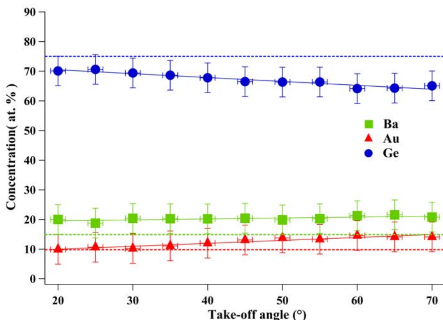
FIGURE 3.3: Elemental near-surface composition measured as a function of the photoelectrons take-off angle for the sample annealed at 833 K. The measurements at 70^\circ are more surface sensitive than those implemented at 20^\circ . The dashed lines correspond to bulk composition, while the solid lines are linear fit to data points and are only a guide for the eyes.
