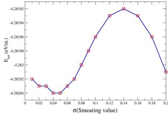
FIGURE B.5: Total energy of bulk \text{Ba}_8\text{Au}_6\text{Ge}_{40} as a function of a smearing parameter ( \sigma ) in the range [0.01 - 0.2].
