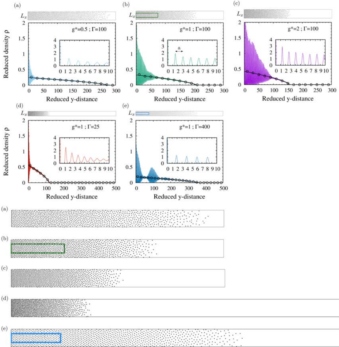
Figure 6.4: Monte Carlo simulation density profiles with magnetic coupling \Gamma = 100 for different values of the gravity parameter (a) g^* = 0.5 , (b) g^* = 1 , and (c) g^* = 2 . Three additional profiles at prescribed g^* = 1 with (d) \Gamma = 25 and (e) \Gamma = 400 . are also displayed. The thick (black) line is the LDA theoretical prediction, see Eq. (6.13). The circles represent the smoothed density profiles, see also text. The insets show a magnified view. Accompanying microstructure snapshots are sketched on the top of panels (a)-(e) and magnified versions are shown at the bottom half of the figure. The unit length is \ell_s^{(\text{ref})} for the whole figure.
