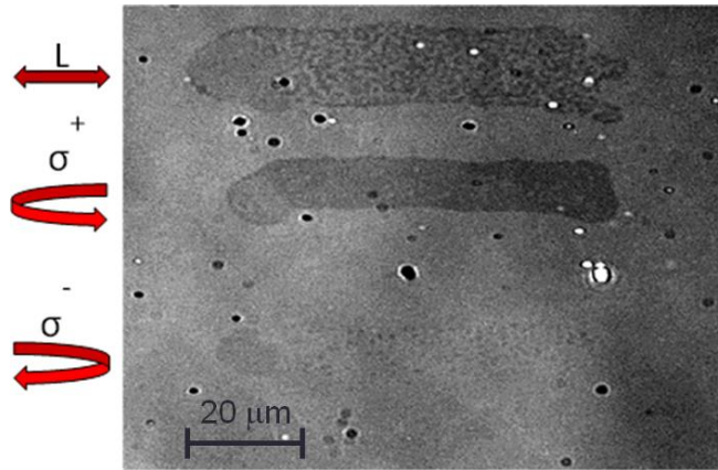
Figure III.5: Faraday imaging after the sweeping of a right-circularly ( \sigma^- ), a linear L and a left-circularly ( \sigma^+ ) polarized laser beam over the Glass/Ta(3nm)/Pt(5nm)/[Pt(2nm)/Co(0.6nm)] 2 /IrMn(8nm)/Pt(3nm) sample at a sweeping speed of 5 \mu m/s. For all exposures to the laser the fluence was 8.9 mJ/cm 2 . The magnetization of the sample has been saturated in the -z direction before the sweeping of the laser.
