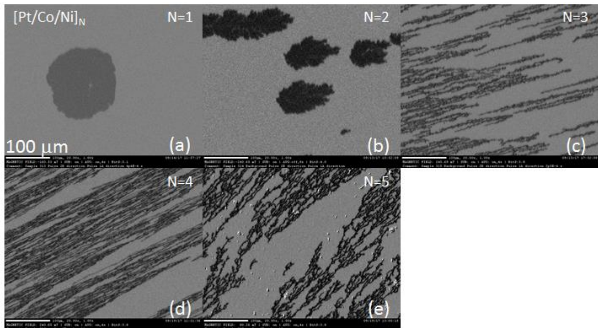
Figure IV.2: MOKE images of domain expansion in the [Pt/Co/Ni] N samples with a) N=1, b) N=2, c) N=3, d) N=4, e) N=5. The resulting domains are either bubbles (a), dendritic (b) or stripes (c-e).
