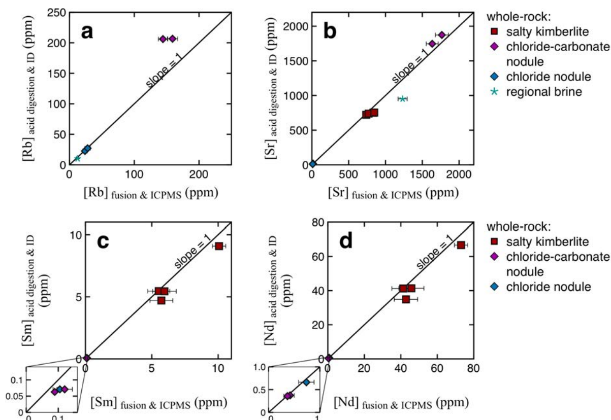
437 438 Figure 6: Rb (a), Sr (b), Sm (c) and Nd concentrations (d) of whole-rock samples measured 439 by acid digestion and isotopic dilution (ID) compared to the concentrations measured by 440 fusion and ICP-MS at the SARM laboratory. Concentrations obtained by the two methods are 441 within uncertainty, except for the Rb-contents of chloride-carbonate nodules due to their non- 442 conventional matrix compositions (Rb-rich alkali-carbonate).
