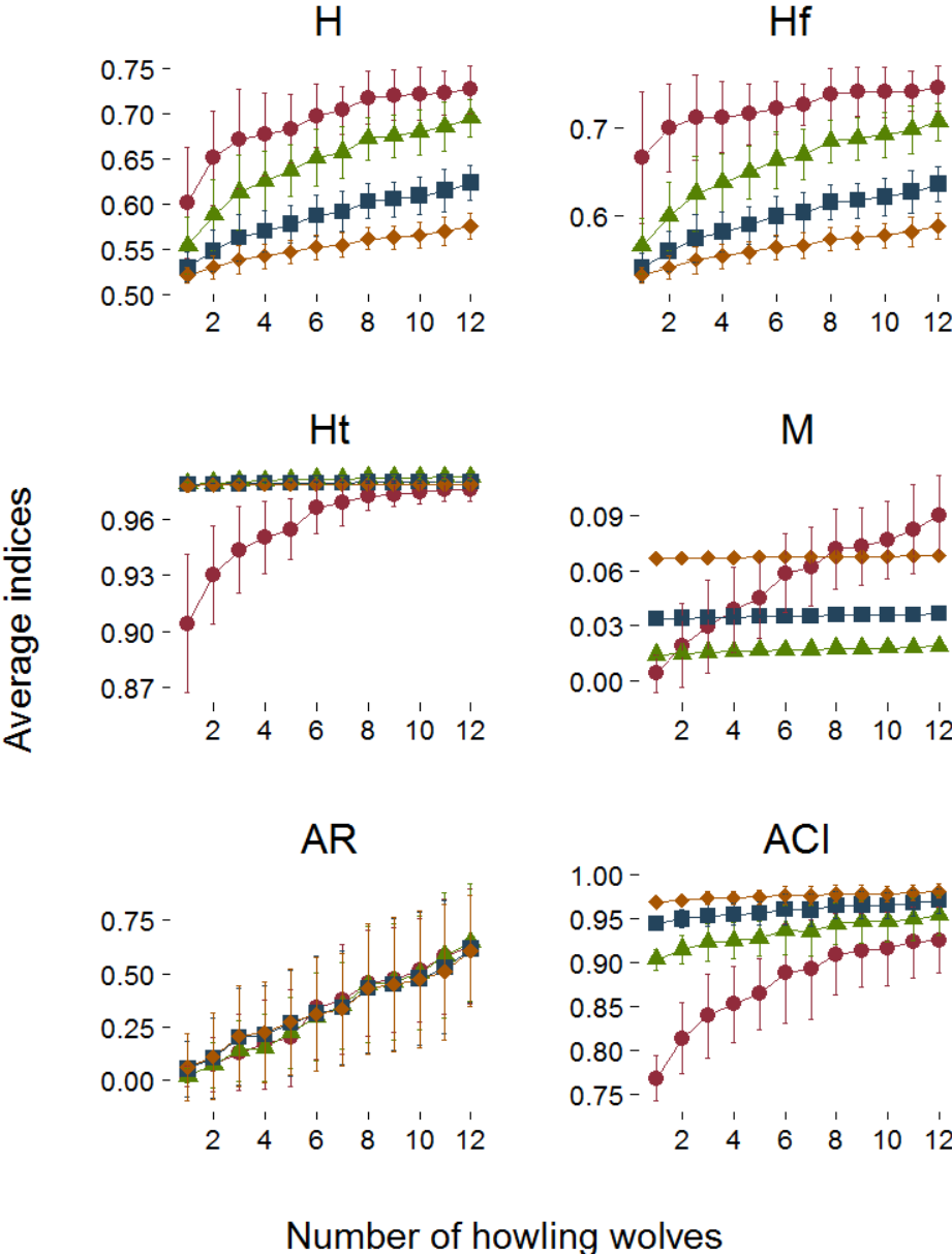
Figure 6: Relationship between the average indices ( \pm SD) and the number of howling wolves in artificial solos and choruses according to different signal-to-noise ratios (SNRs). Red circles: Control (T0) with artificial solos and choruses without any background noise. Green triangles: Treatment T1 (T0 mixed with background noise with a high SNR). Blue squares: treatment T2 (T0 mixed with background noise with a medium SNR). Orange diamonds: treatment T3 (T0 mixed with background noise with a low SNR). All indices for all treatments remained significantly positively correlated with the number of howling wolves (Spearman’s rank correlation coefficient, P < 0.01 ).
