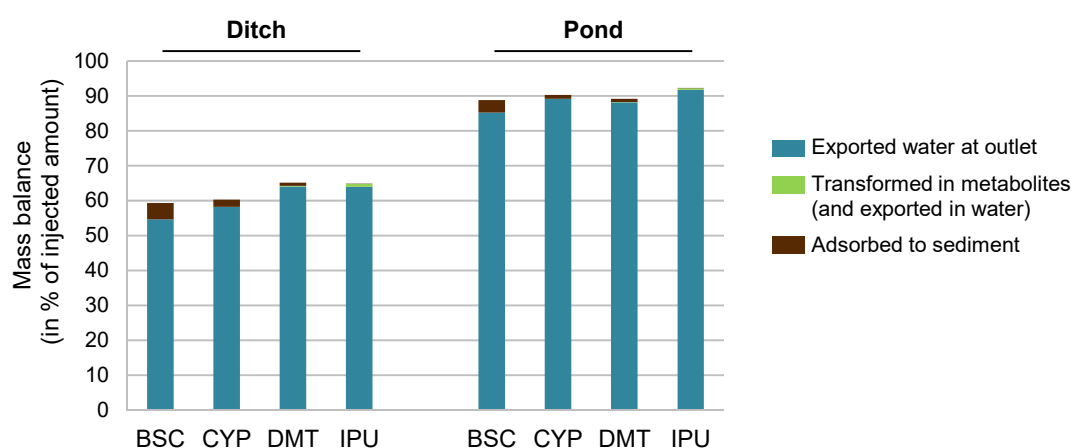
Figure D-5: Mass balance during a complete drainage period (alternating phases of high-, low- and no-flow) for the ditch and the pond over 62 days.
