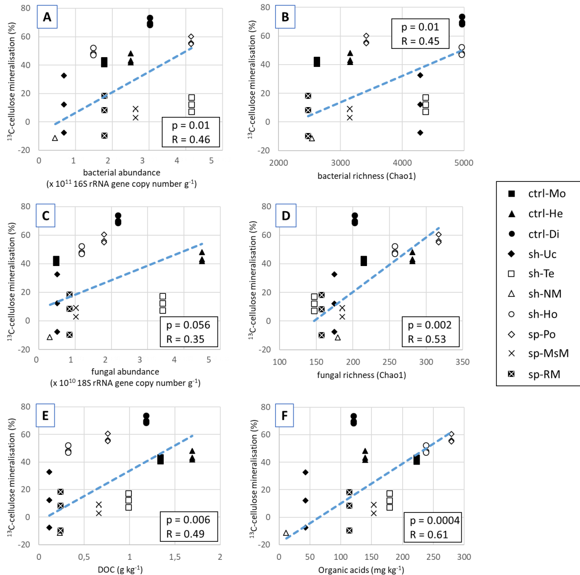
Figure 6.2. Correlation between the percentage of dissipated 13 C-cellulose mineralisation and biotic/abiotic factors measured on initial soils. Correlation with bacterial abundance and community richness (A and B), with fungal abundance and community richness (C and D), and dissolved organic carbon (DOC) and organic acid contents (E and F). 13 C-cellulose mineralisation value of the second replicate for sh-NM soil (i.e. -122.8%) was excluded from graphs but included in the correlation analysis.
