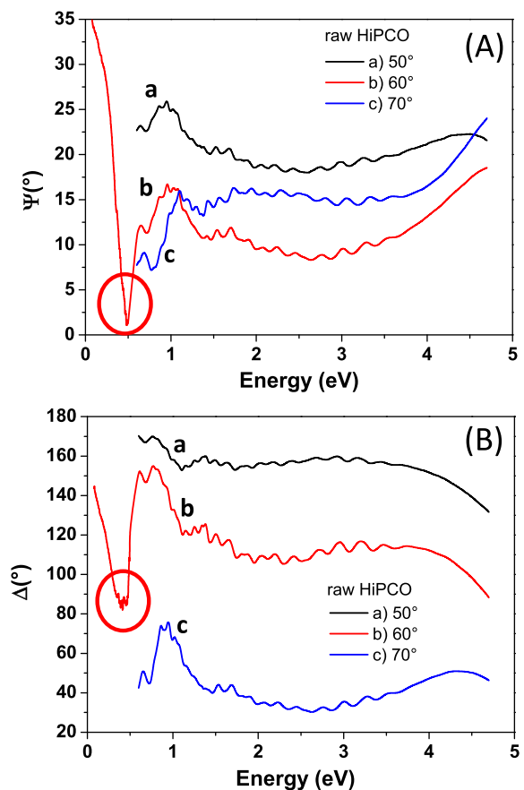
Fig. 7. Spectroscopic ellipsometric angles \Psi and \Delta for raw HiPCO CNTs at three different incident angles. The red circles indicate the connecting points of IR and NIR-visible-UV data. (A colour version of this figure can be viewed online.)
