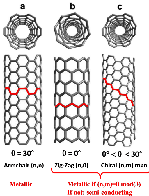
Figure 5: the three main types of possible structures for CNTs: the chair structure (armchair), the zig-zag structure and the chiral structure, with the associated values of the chirality angle \theta and chiral indices (n, m) .
