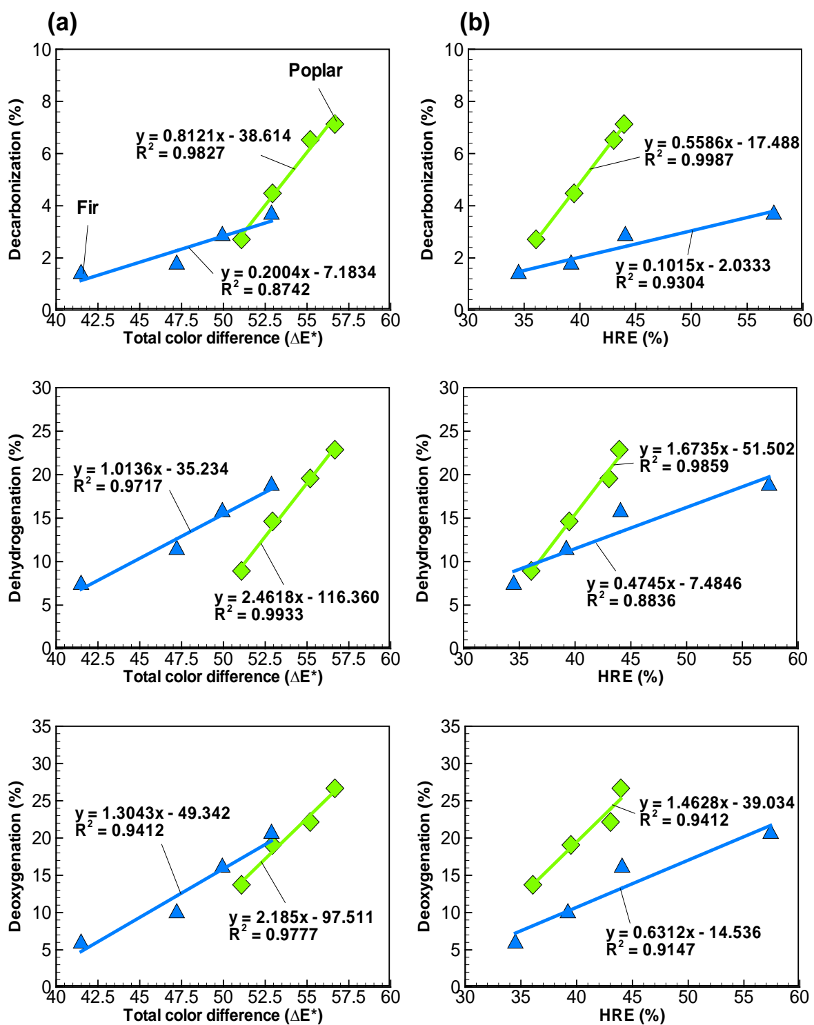
Fig. 4-17. Profiles and linear regressions of (a) total color difference ( \Delta E^* ) and (b) hygroscopicity reduction extent (HRE) versus decarbonization, dehydrogenation, and deoxygenation.
