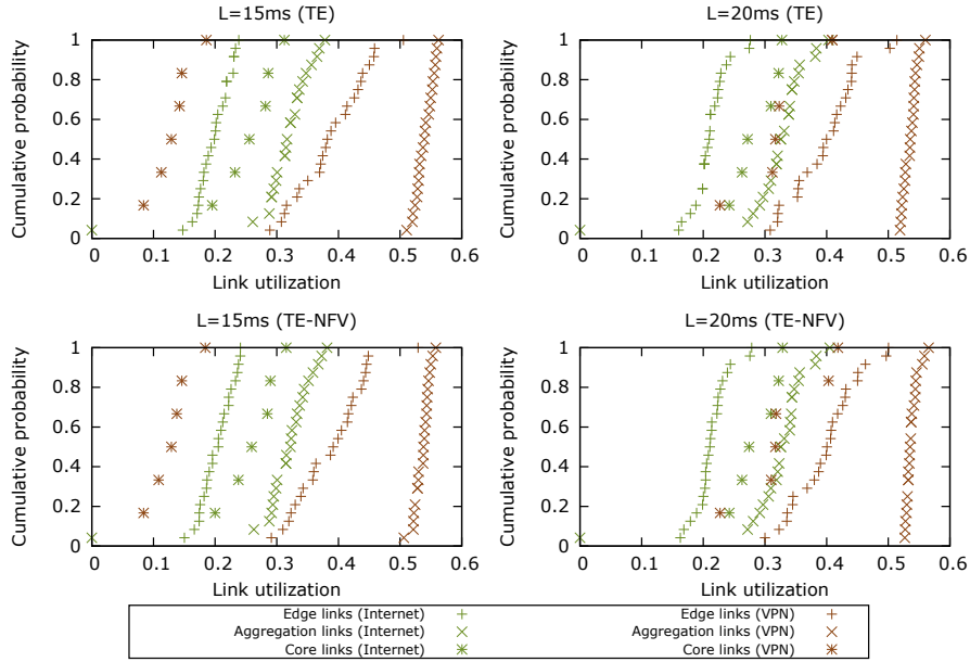
Figure 3.6 – Link utilization empirical CDFs (standard case).
