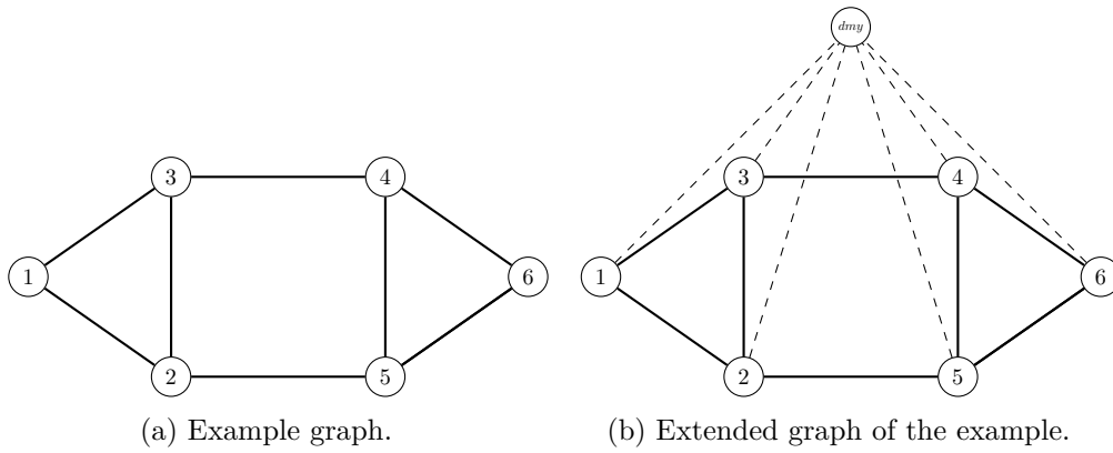
Figure 5.1 – The graph extension operated by model \text{SP}^{\text{MD}} .
