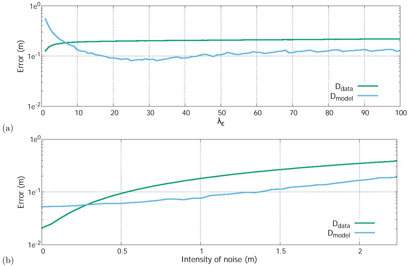
Figure 3.15: Sensitivity of the proposed method to the noise and the energy weight \lambda_\epsilon . (a) The intensity of noise is fixed to 1m, and \lambda_\epsilon varies. (b) The weight \lambda_\epsilon is fixed to 30 and the intensity of noise varies.
