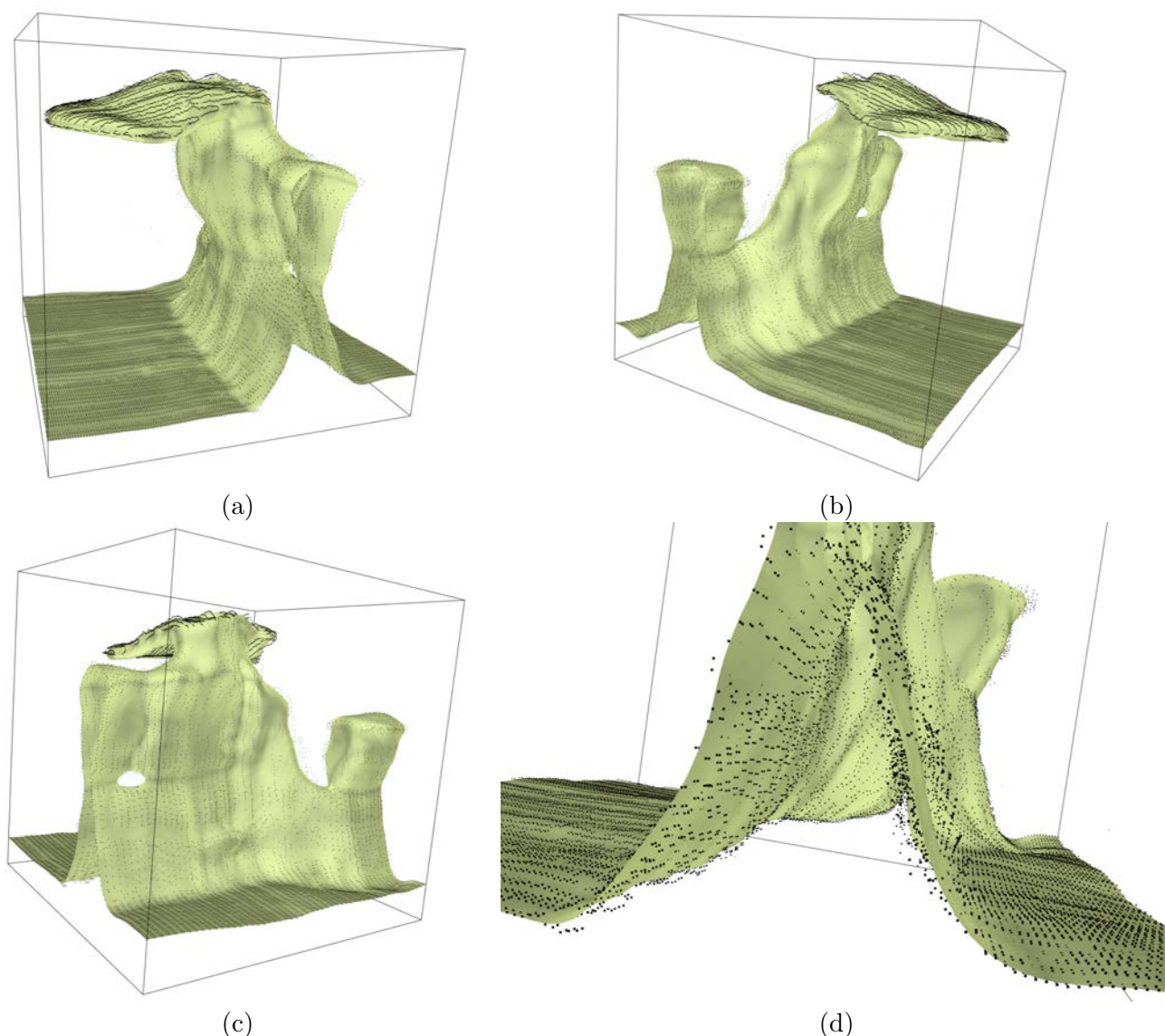
Figure 6.4: 3D salt surface constructed with this thesis's framework on a point set issued from the interpretation of parallel slides on an analogue sandbox model of the Nordkapp basin. (a), (b) and (c) Three different points of view of the constructed surface, and (d) Zoom showing the noise in the data point set.
