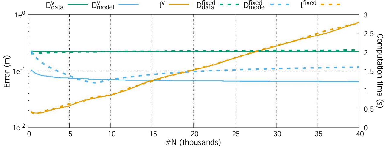
Figure 3.17: Sensitivity of the proposed method to the number of computation nodes \#N on the data points from Figure 3.14. The distances D_{model}^{\nu} , D_{data}^{\nu} and computation times t^{\nu} were computed with a \lambda_{\epsilon} dependent on the discretization (i.e., \lambda_{\epsilon} = 30\sqrt{\nu} ). The distances D_{model}^{fixed} , D_{data}^{fixed} and computation times t^{fixed} were computed with a \lambda_{\epsilon} independent of the discretization (i.e., fixed to \lambda_{\epsilon} = 95 \Leftrightarrow 30\sqrt{\nu} when \#N = 10,000 ).
