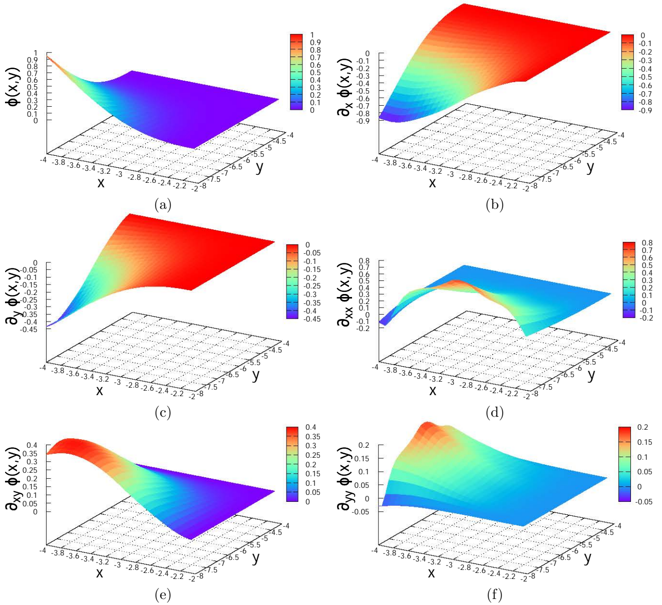
Figure H.6: 2D plots of the MLS functions and their derivatives on a corner node ( \bar{\mathbf{p}} = \{-4, -4\} ) of Figure H.4.
